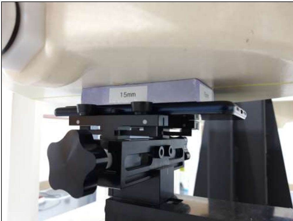
E.2.2) Body-Worn_Rear (15 mm)
