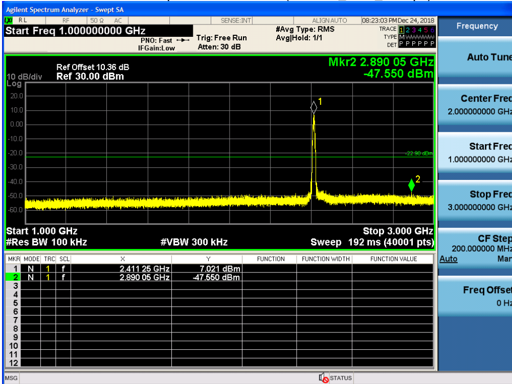
Conducted Spurious Emission (802.11b_Ch.1_2 Mbps)
