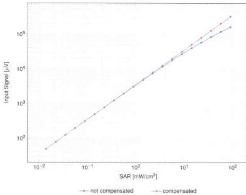
Dynamic Range f(SAR_{head}) (TEM cell, f_{eval} = 1900\text{MHz} )
