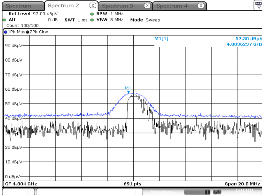
Radiated Spurious Emissions plot – Average & Peak Result (GFSK, Ch.0 2nd Harmonic, X-H)
