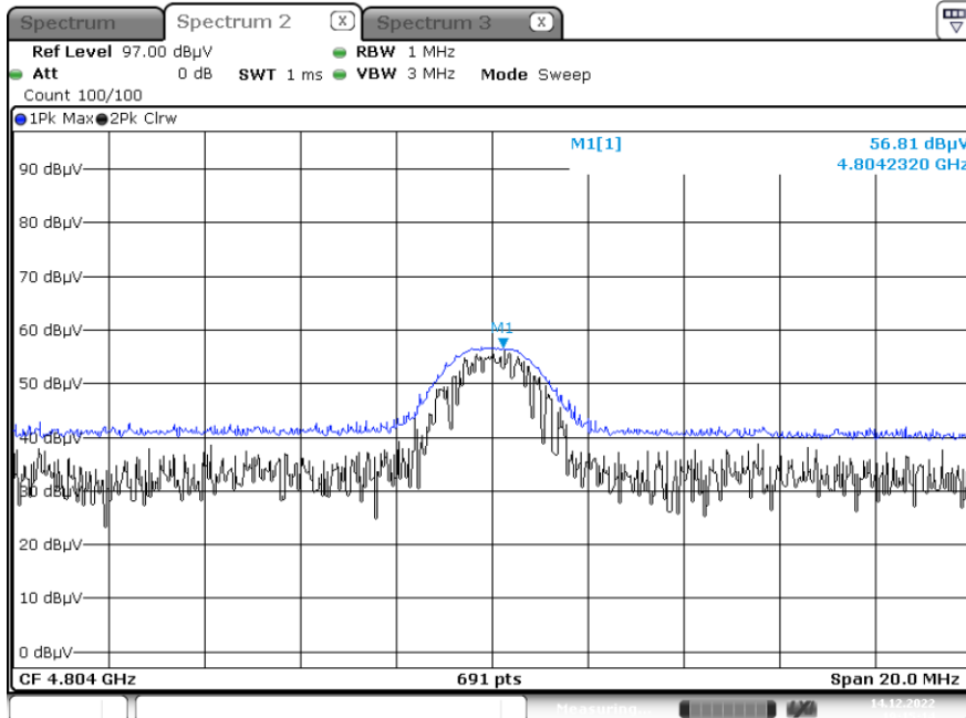
Radiated Spurious Emissions plot – Average & Peak Result (2nd Harmonic, X-H)
