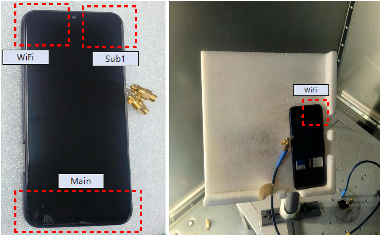
- Return Loss & VSWR Test, Photo #2
