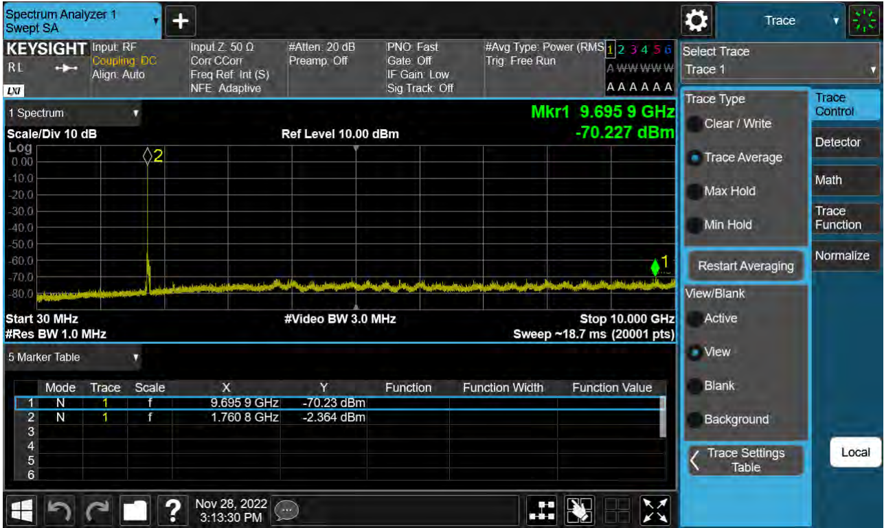
Sub6 n66. Conducted Spurious Plot_1 (354000ch_20 MHz_BPSK_RB 1_1)
