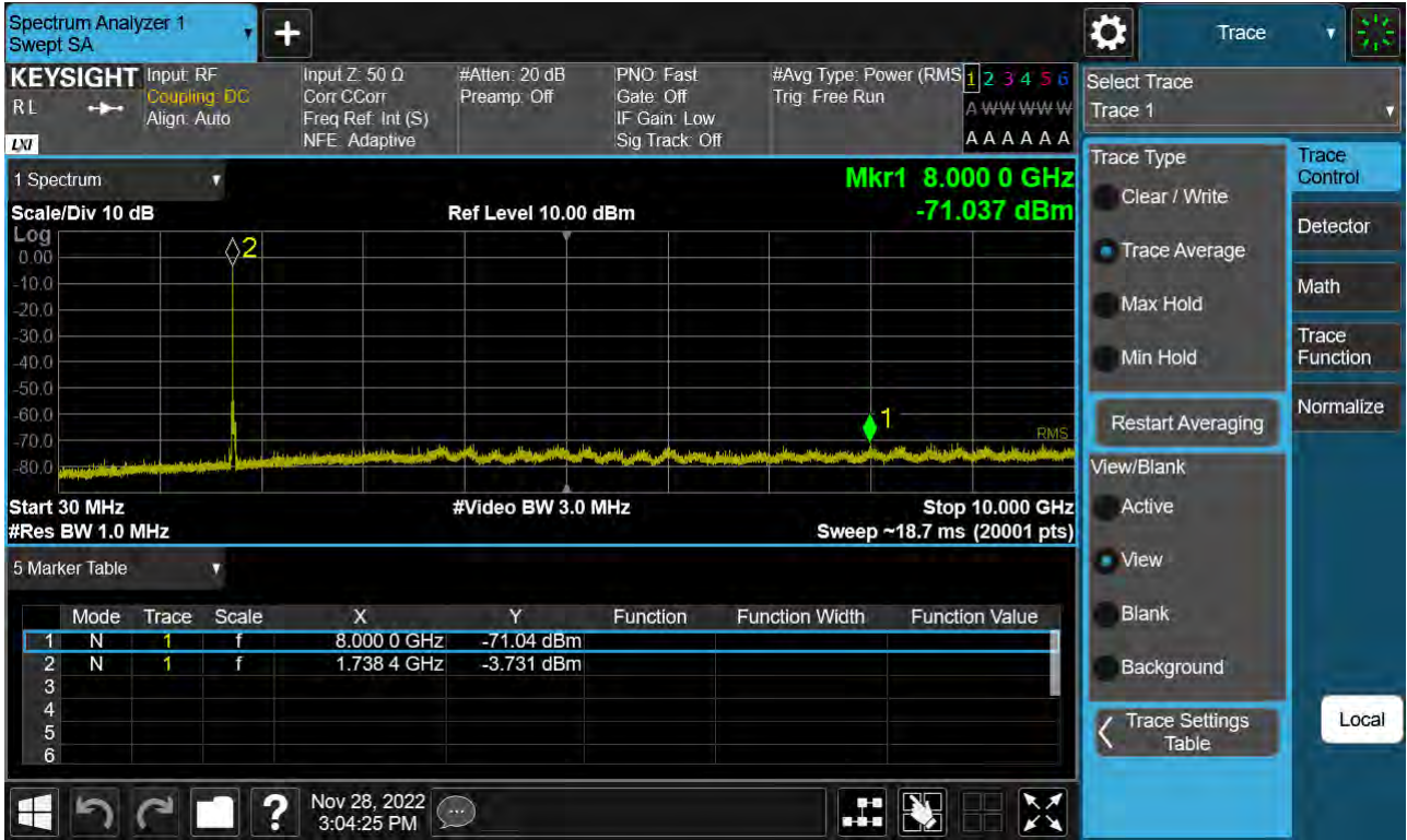
Sub6 n66. Conducted Spurious Plot_1 (349000ch_15 MHz_BPSK_RB 1_1)
