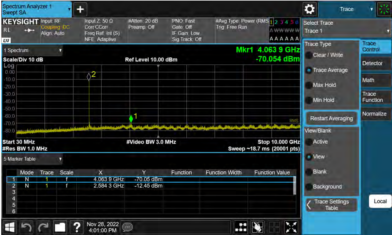
Sub6 n41. Conducted Spurious Plot 1 (20 MHz Ch.518598 BPSK RB 1)
