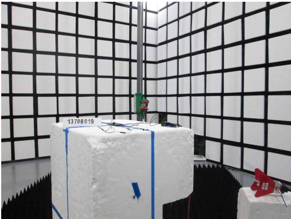
RADIATED BACK PHOTO (ABOVE 1GHz)
