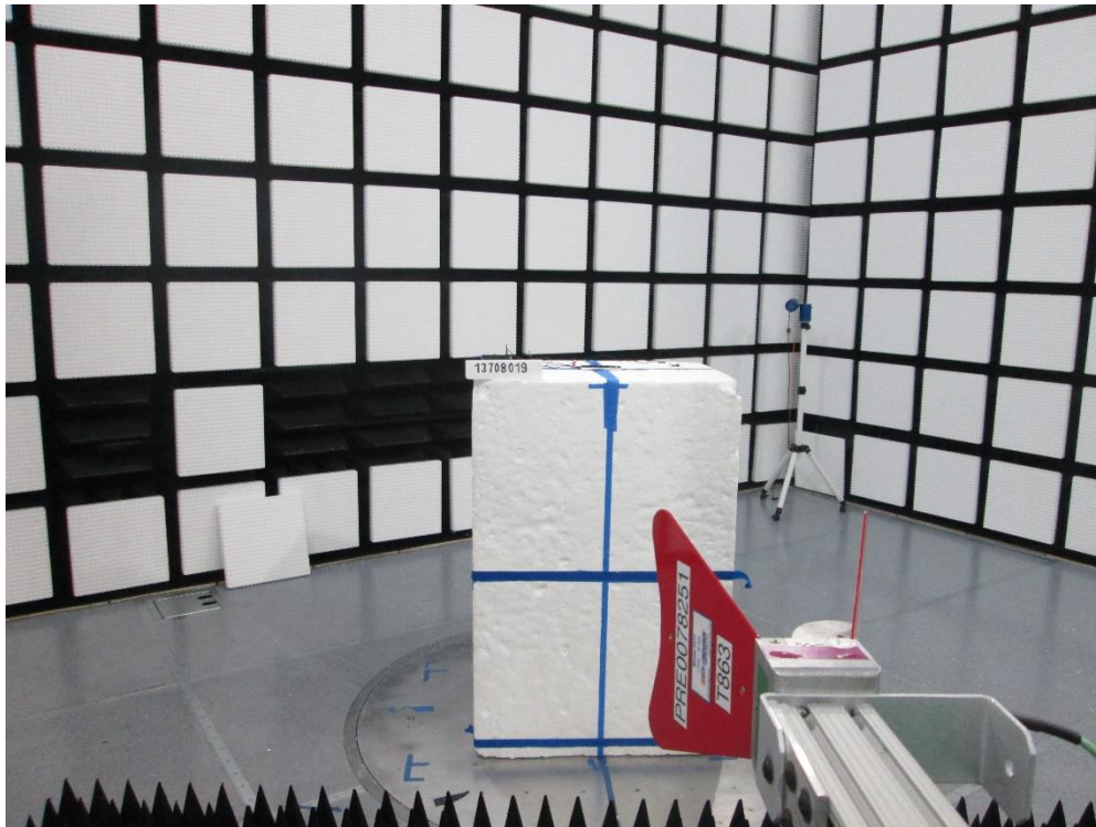
RADIATED FRONT PHOTO (ABOVE 1GHz)
