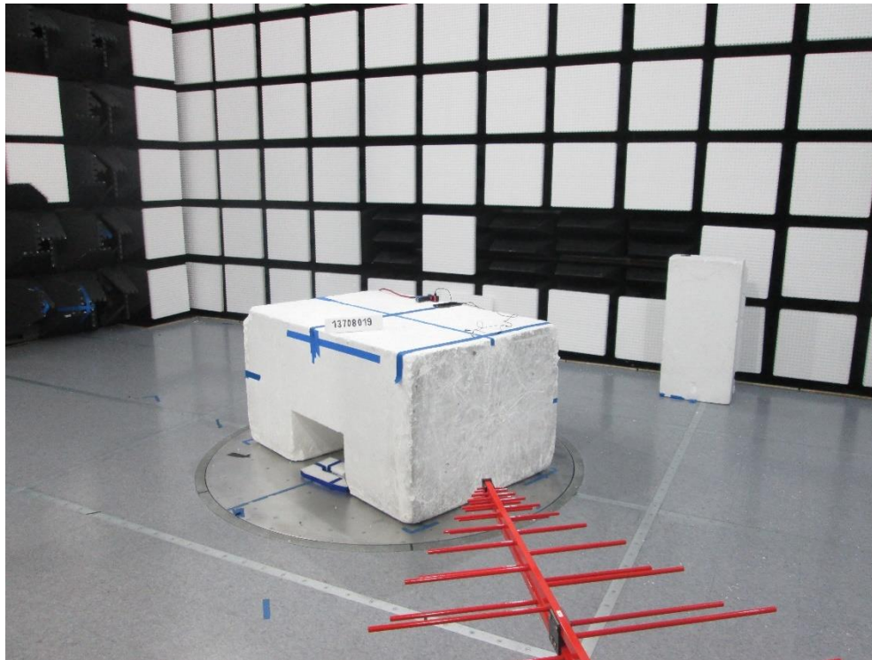
RADIATED FRONT PHOTO (BELOW 1GHz)
