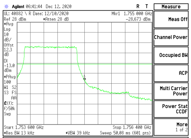
LTE B4 1.4MHz QPSK High Channel RB6-0
