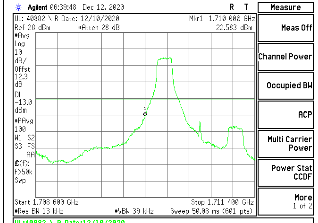
LTE B4 1.4MHz 16QAM Low Channel RB1-0
