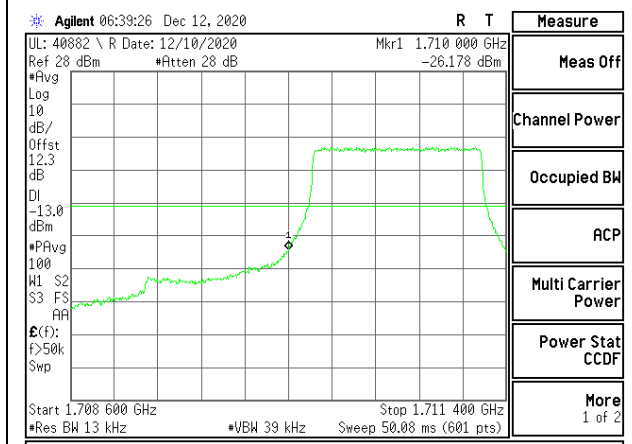
LTE B4 1.4MHz QPSK Low Channel RB6-0
