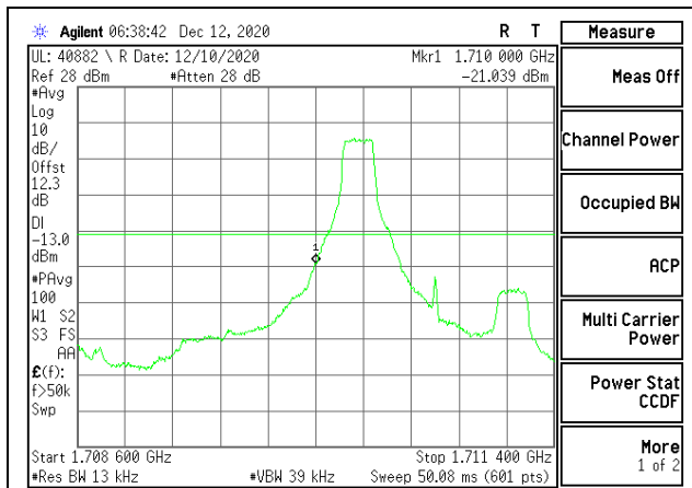
LTE B4 1.4MHz QPSK Low Channel RB1-0
