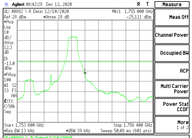
LTE B4 1.4MHz 16QAM High Channel RB1-5
