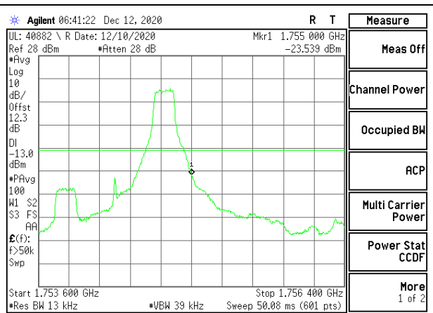
LTE B4 1.4MHz QPSK High Channel RB1-5
