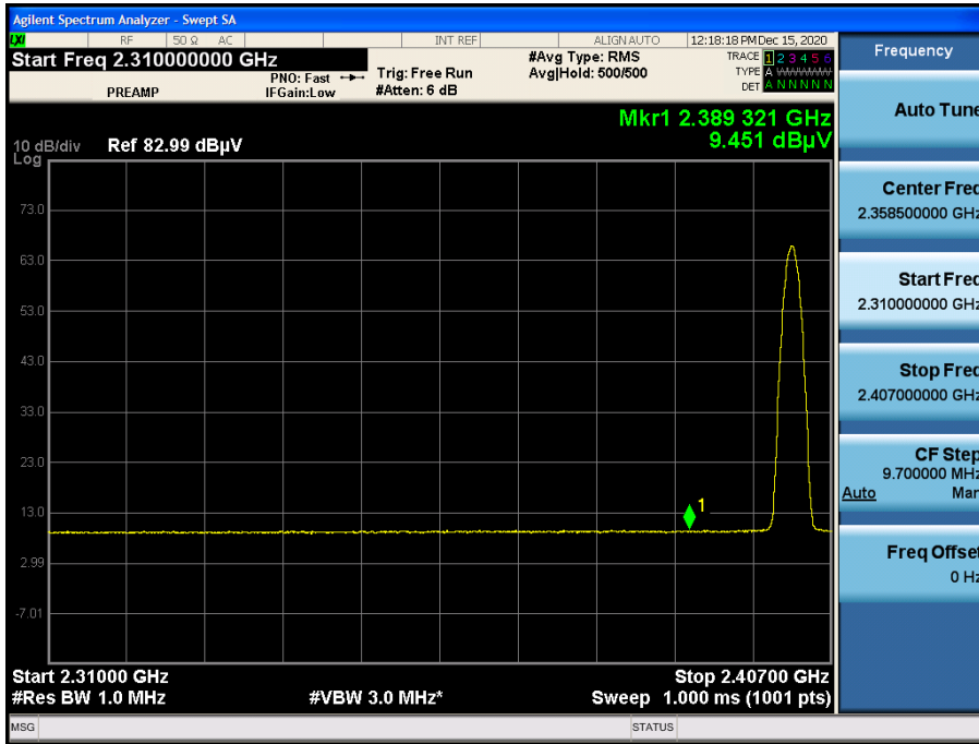
Radiated Restricted Band Edges plot – Peak Reading (Ch.0, Z-V)
