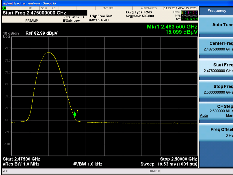
Radiated Restricted Band Edges plot – Average Reading (8DPSK, Ch.78, Z-V)
