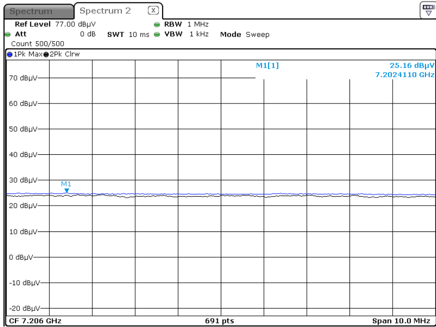
Radiated Spurious Emissions plot – Peak Reading (8DPSK, Ch.0 3rd Harmonic, Y-H)
