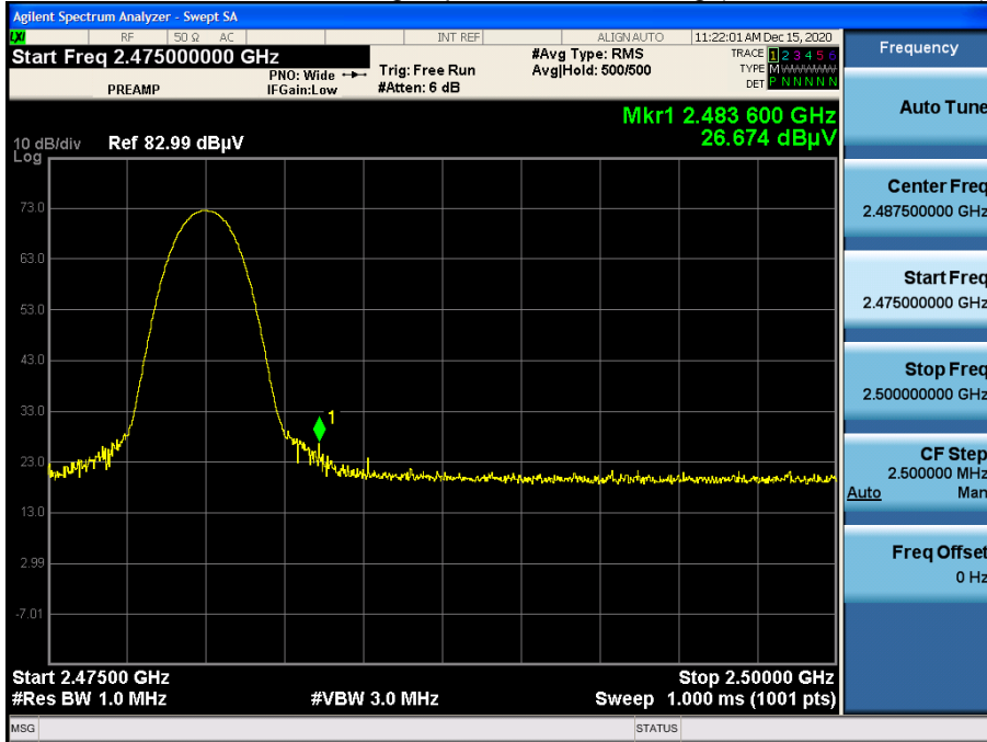
Radiated Restricted Band Edges plot – Peak Reading (8DPSK, Ch.78, Z-V)
