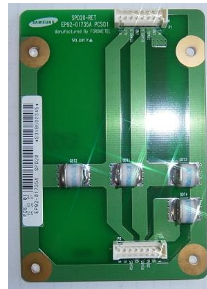
SPD20-RET (Lightning Protection PBA for RET Line)
