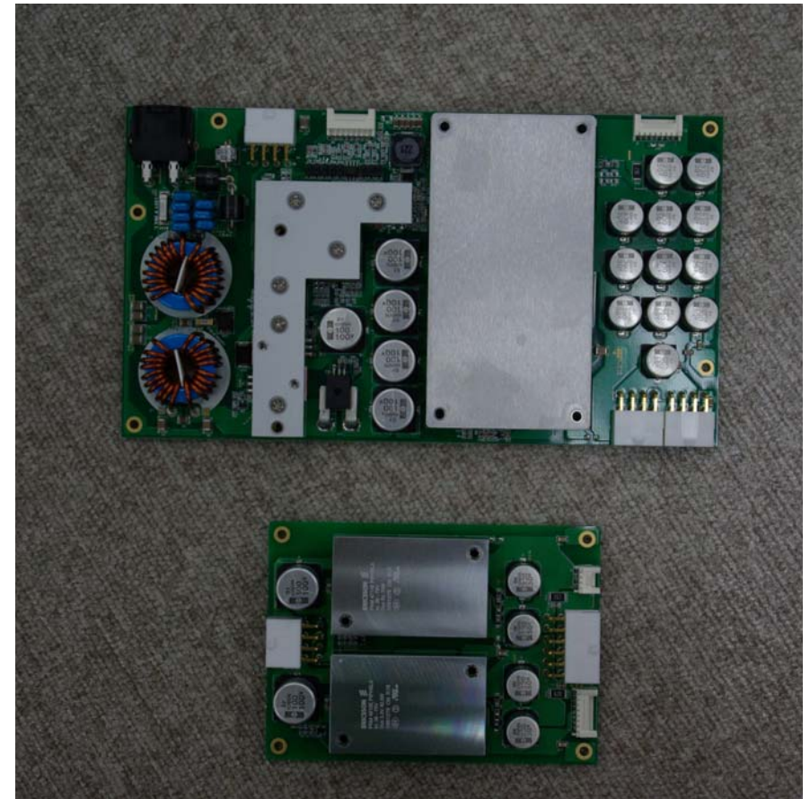
MDCDC(back)
