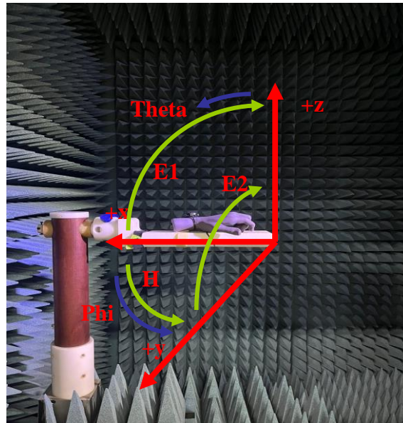
Figure 4: Geometry for SM-L315U for Radiation patterns.
