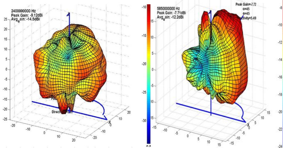
<Smart Watch mounted typical measurements>
