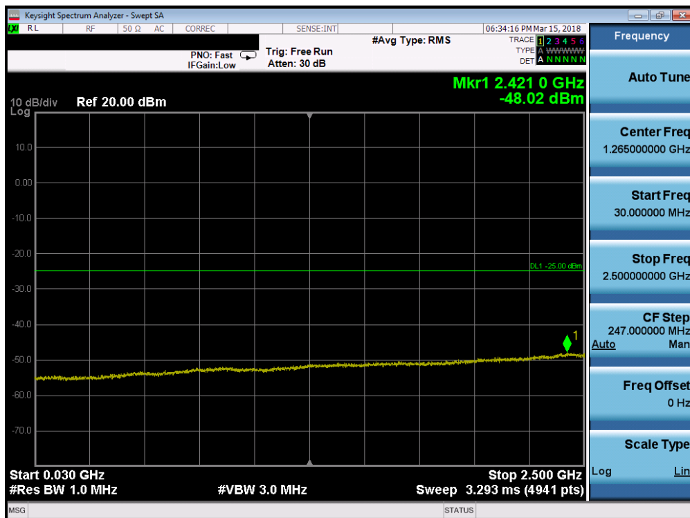
Plot 7-78. Conducted Spurious Plot (Band 7 - 10.0MHz QPSK - RB Size 1, RB Offset 0 - Mid Channel)
