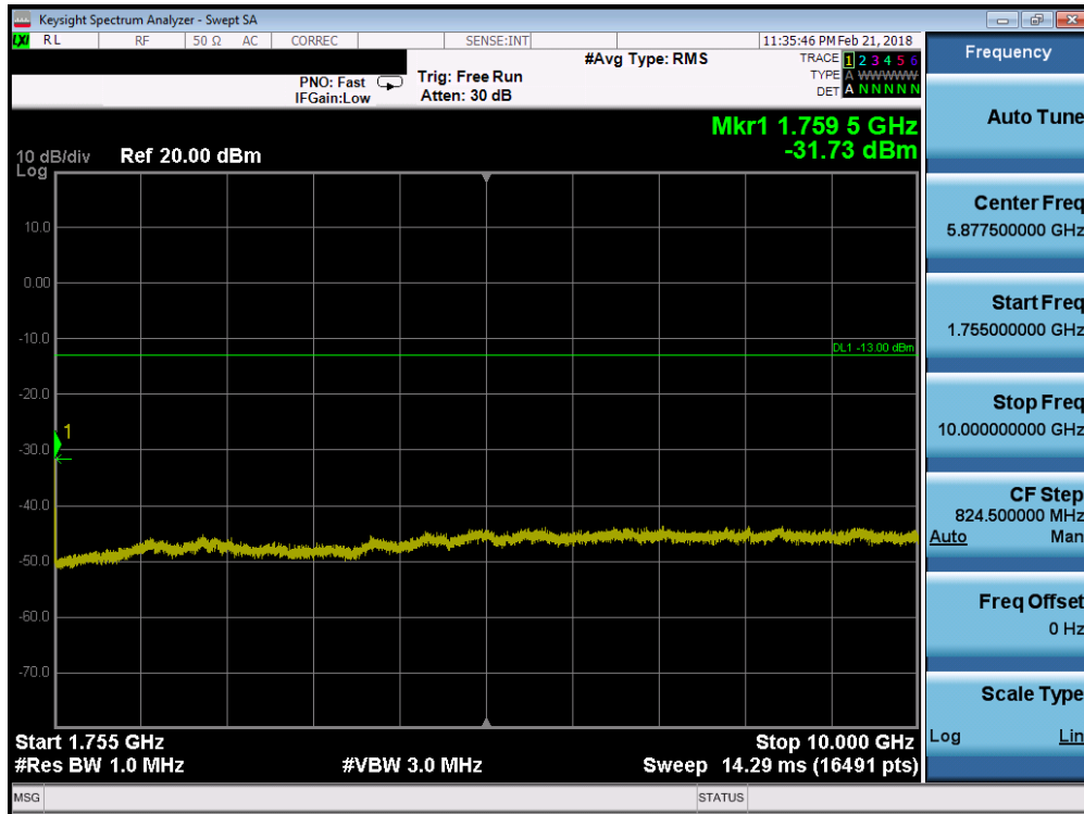
Plot 7-61. Conducted Spurious Plot (Band 4 - 20.0MHz QPSK - RB Size 1, RB Offset 0 - Mid Channel)
