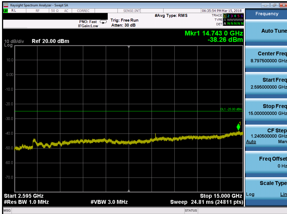
Plot 7-82. Conducted Spurious Plot (Band 7 - 10.0MHz QPSK - RB Size 1, RB Offset 0 - High Channel)
