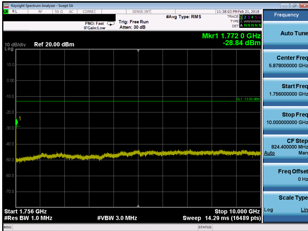
Plot 7-64. Conducted Spurious Plot (Band 4 - 20.0MHz QPSK - RB Size 1, RB Offset 0 - High Channel)
