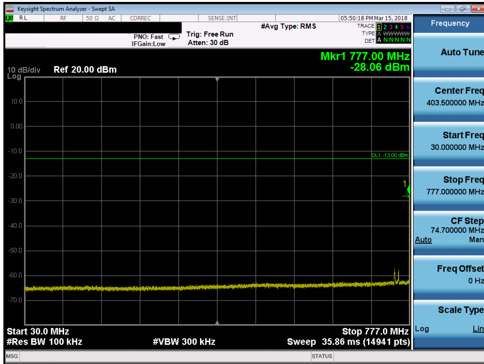
Plot 7-45. Conducted Spurious Plot (Band 13 - 10.0MHz QPSK - RB Size 1, RB Offset 0)
