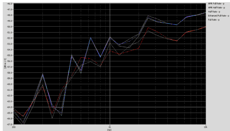
Figure 4-14 Vocoder Analysis for ABM Noise for GSM
