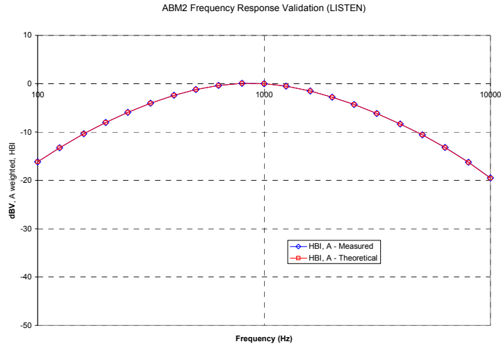
Figure 4-9 ABM2 Frequency Response Validation
