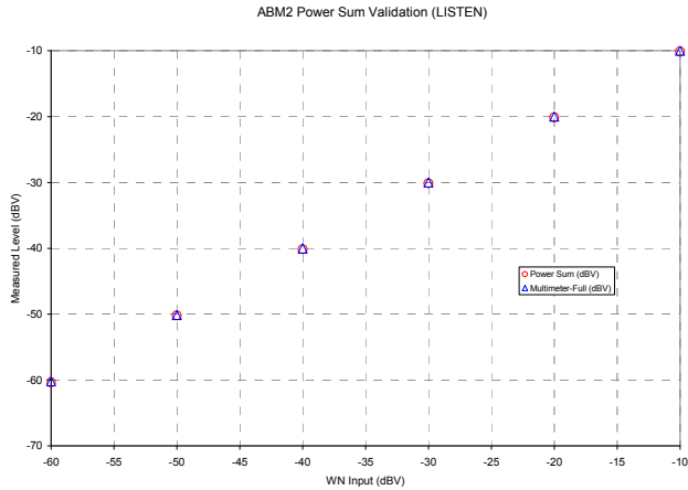
Figure 4-11 ABM2 Power Sum Validation
