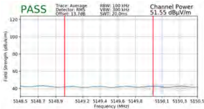
Plot 7-86. Radiated Lower Band Edge Plot (Average – UNII Band 1)
