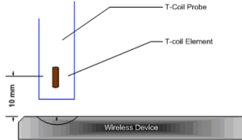
Figure 4-12 Measurement Distance
