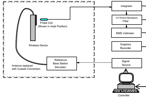
Figure 4-15 Audio Magnetic Field Test Setup
