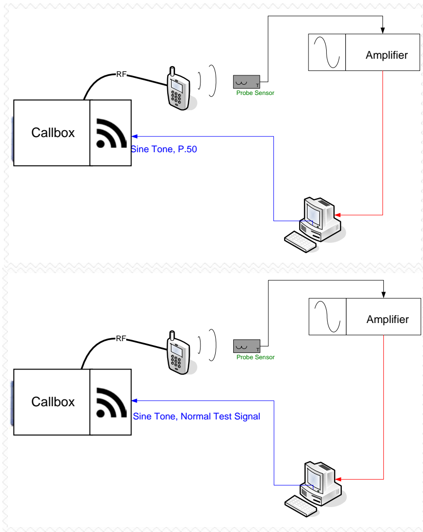
Figure 4-2 T-Coil Test Setup
