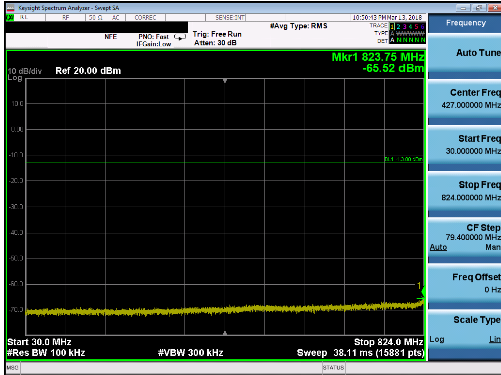
Plot 7-72. Conducted Spurious Plot (Band 5 - 3.0MHz QPSK - RB Size 1, RB Offset 0 - High Channel)
