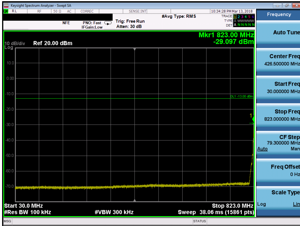
Plot 7-66. Conducted Spurious Plot (Band 5 - 3.0MHz QPSK - RB Size 1, RB Offset 0 - Low Channel)
