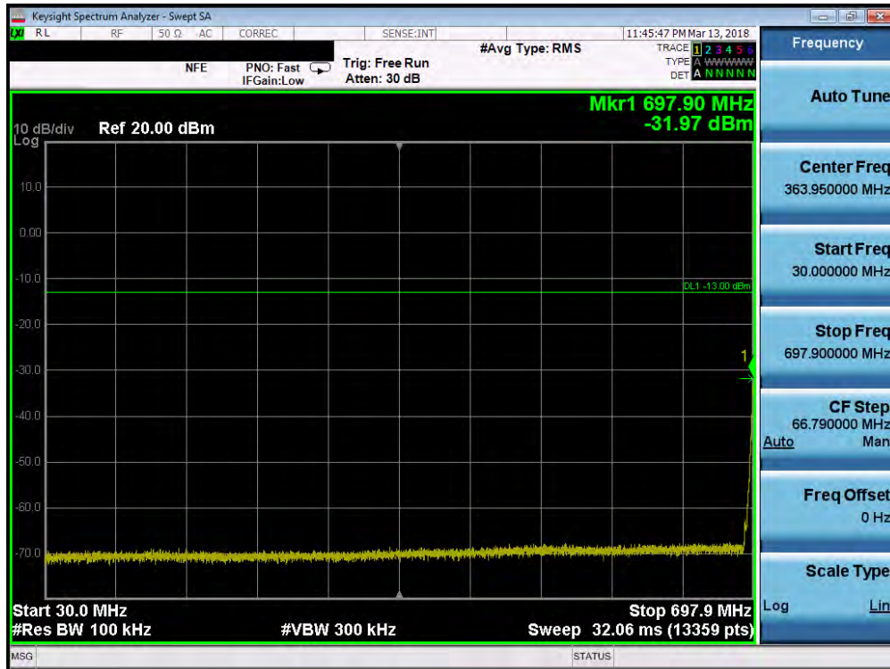
Plot 7-57. Conducted Spurious Plot (Band 12 - 3.0MHz QPSK - RB Size 1, RB Offset 0 - Low Channel)
