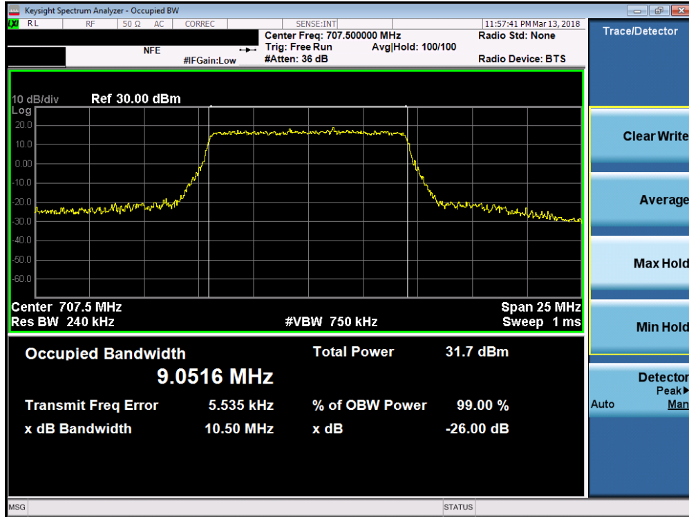
Plot 7-55. Occupied Bandwidth Plot (Band 12 - 10.0MHz QPSK - Full RB Configuration)
