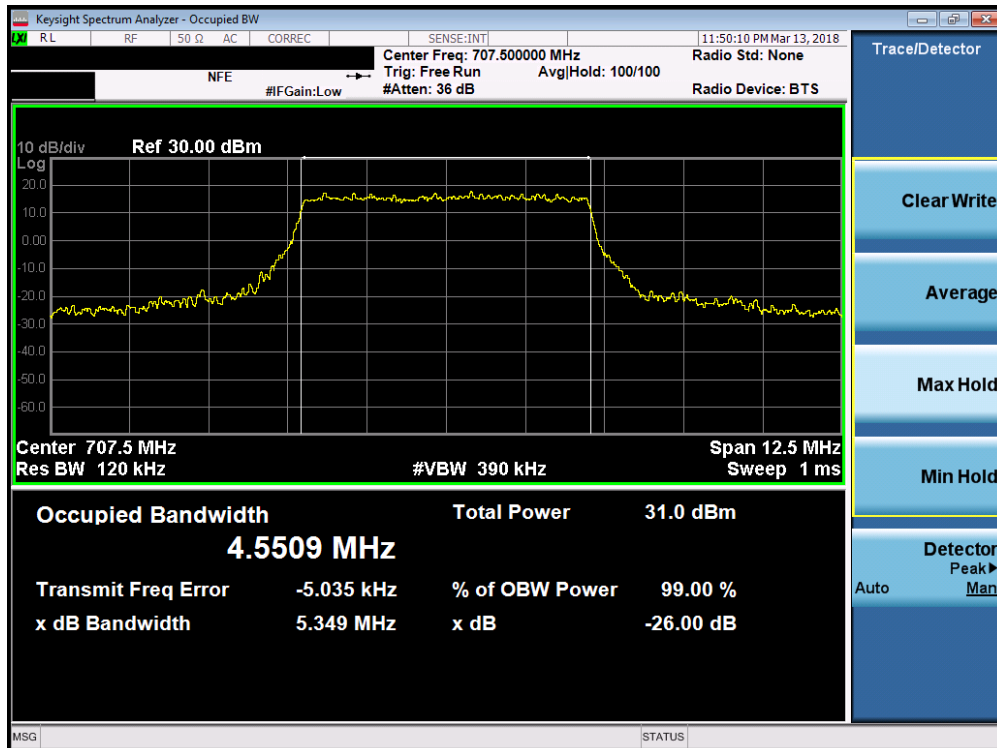
Plot 7-54. Occupied Bandwidth Plot (Band 12 - 5.0MHz 16-QAM - Full RB Configuration)
