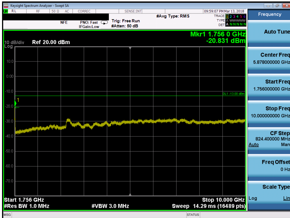
Plot 7-82. Conducted Spurious Plot (Band 4 - 20.0MHz QPSK - RB Size 1, RB Offset 0 - High Channel)
