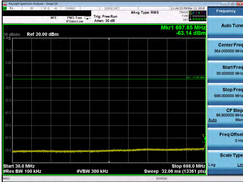
Plot 7-63. Conducted Spurious Plot (Band 12 - 3.0MHz QPSK - RB Size 1, RB Offset 0 - High Channel)
