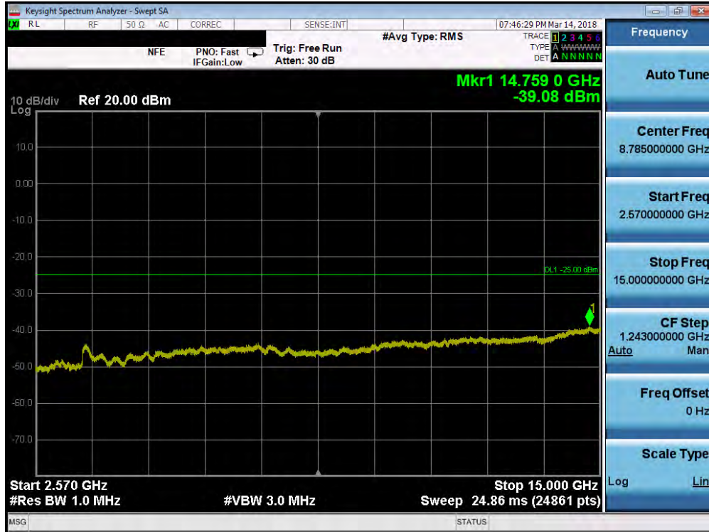
Plot 7-97. Conducted Spurious Plot (Band 7 - 10.0MHz QPSK - RB Size 1, RB Offset 0 - Mid Channel)
