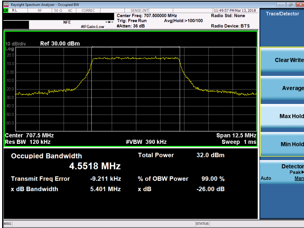
Plot 7-53. Occupied Bandwidth Plot (Band 12 - 5.0MHz QPSK - Full RB Configuration)
