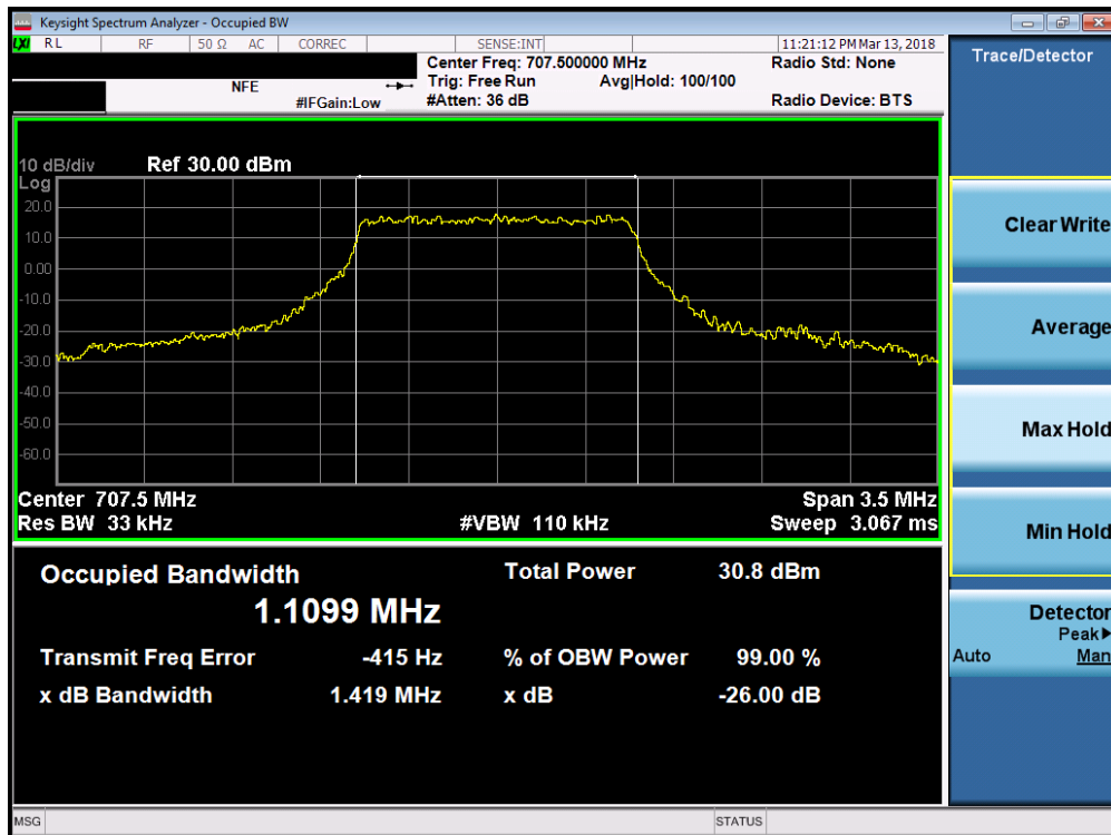
Plot 7-50. Occupied Bandwidth Plot (Band 12 - 1.4.0MHz 16-QAM - Full RB Configuration)
