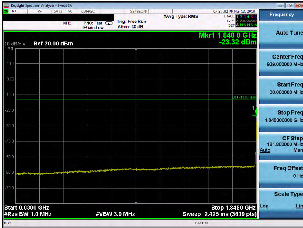
Plot 7-84. Conducted Spurious Plot (Band 2 - 5.0MHz QPSK - RB Size 1, RB Offset 0 - Low Channel)
