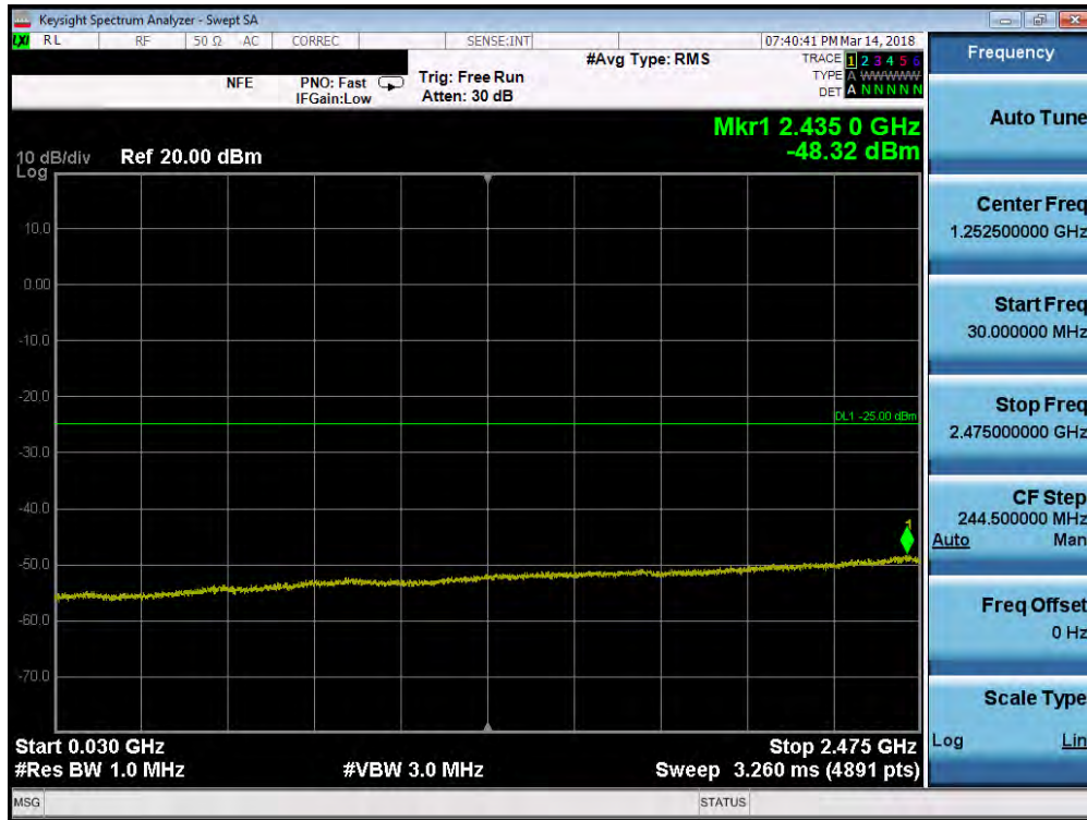
Plot 7-93. Conducted Spurious Plot (Band 7 - 10.0MHz QPSK - RB Size 1, RB Offset 0 - Low Channel)
