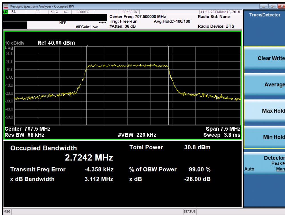
Plot 7-52. Occupied Bandwidth Plot (Band 12 - 3.0MHz 16-QAM - Full RB Configuration)
