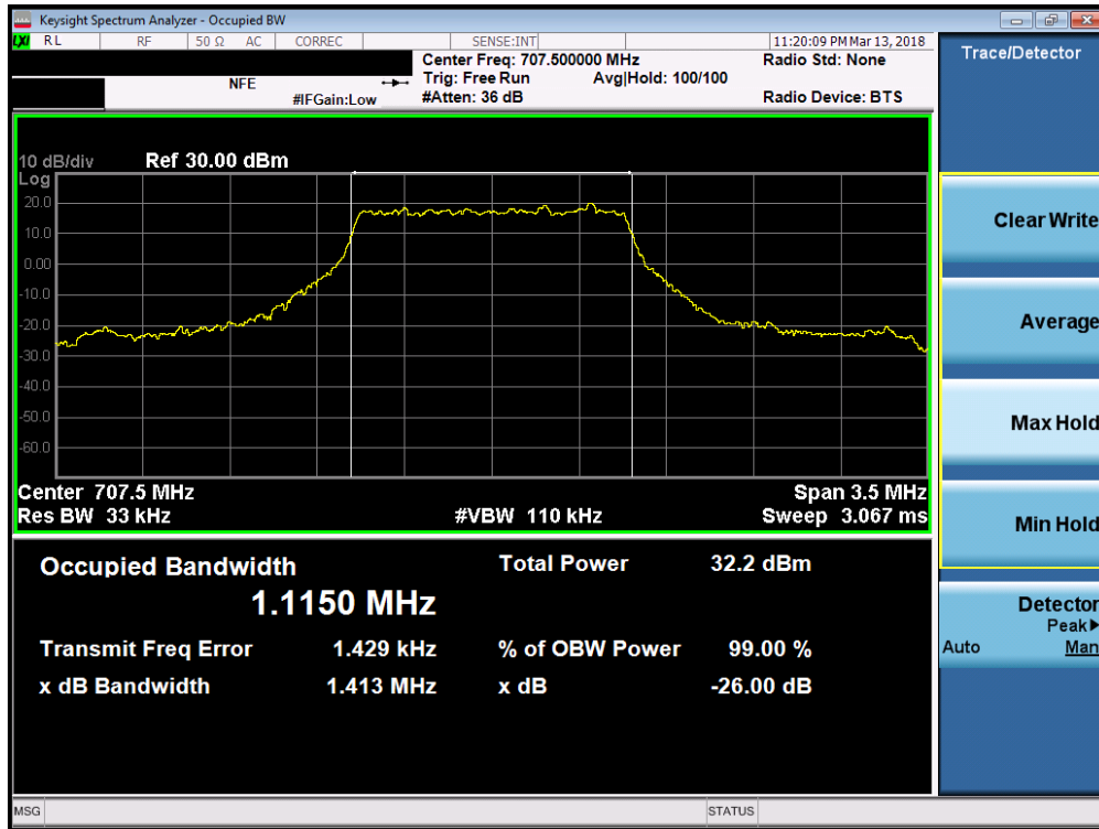
Plot 7-49. Occupied Bandwidth Plot (Band 12 - 1.4.0MHz QPSK - Full RB Configuration)
