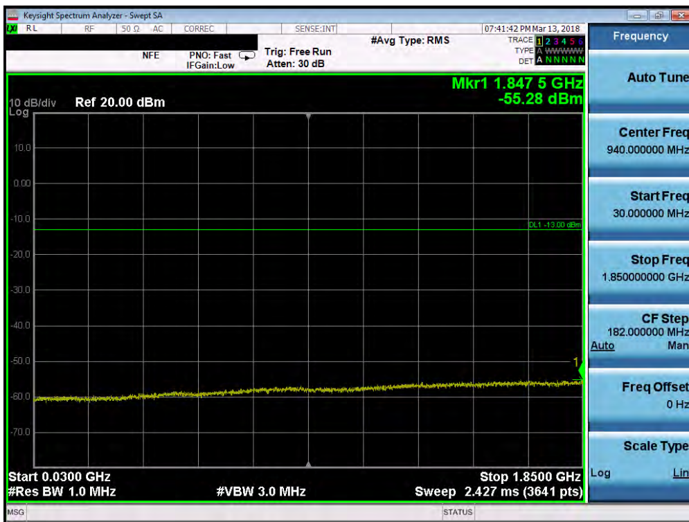
Plot 7-87. Conducted Spurious Plot (Band 2 - 5.0MHz QPSK - RB Size 1, RB Offset 0 - Mid Channel)
