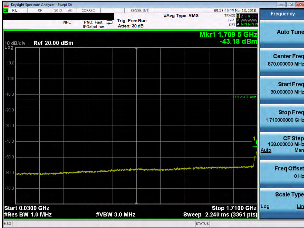
Plot 7-81. Conducted Spurious Plot (Band 4 - 20.0MHz QPSK - RB Size 1, RB Offset 0 - High Channel)
