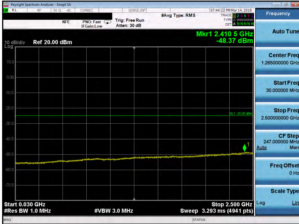
Plot 7-99. Conducted Spurious Plot (Band 7 - 10.0MHz QPSK - RB Size 1, RB Offset 0 - High Channel)
