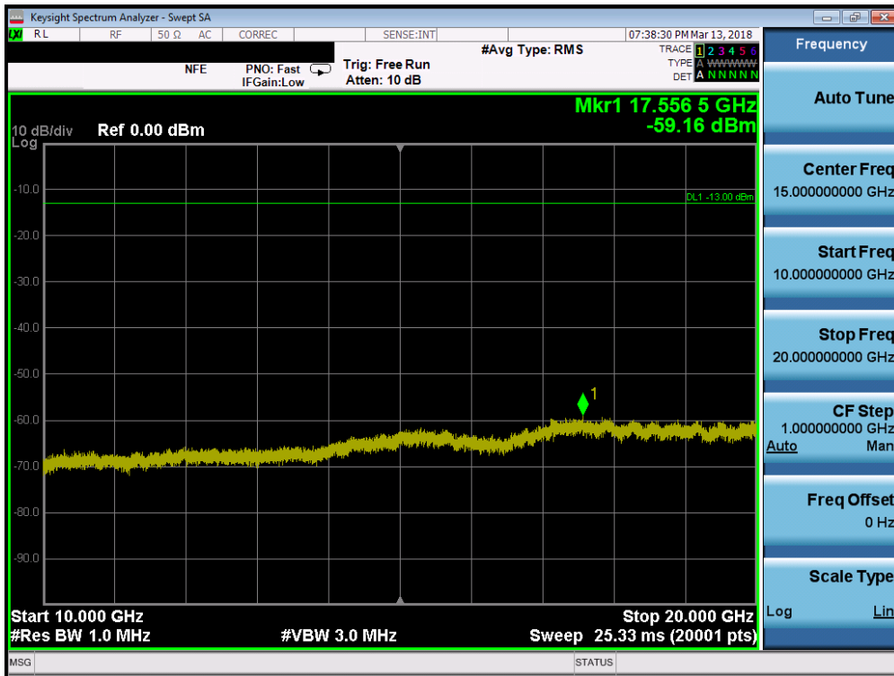
Plot 7-86. Conducted Spurious Plot (Band 2 - 5.0MHz QPSK - RB Size 1, RB Offset 0 - Low Channel)
