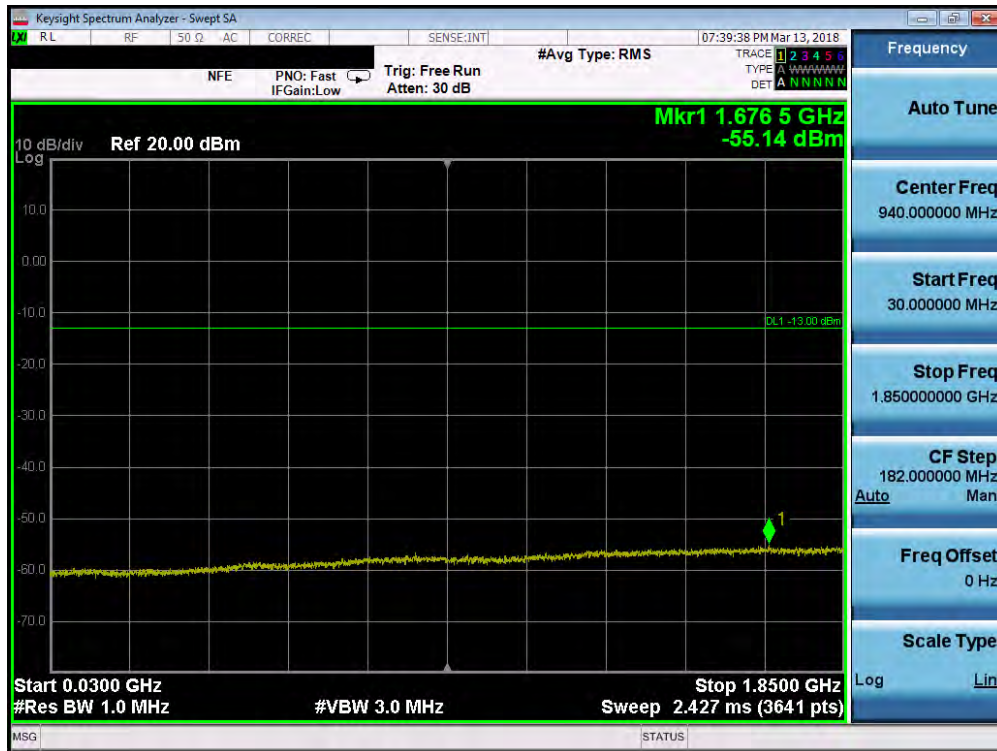
Plot 7-90. Conducted Spurious Plot (Band 2 - 5.0MHz QPSK - RB Size 1, RB Offset 0 - High Channel)
