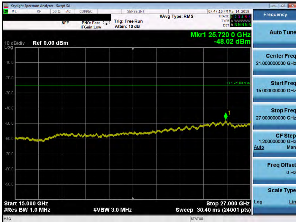
Plot 7-98. Conducted Spurious Plot (Band 7 - 10.0MHz QPSK - RB Size 1, RB Offset 0 - Mid Channel)
