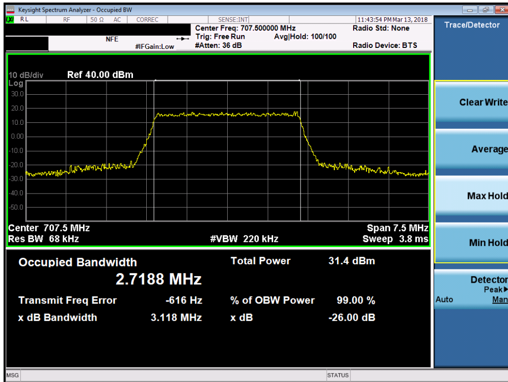
Plot 7-51. Occupied Bandwidth Plot (Band 12 - 3.0MHz QPSK - Full RB Configuration)
