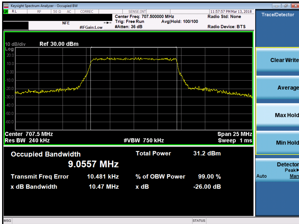
Plot 7-56. Occupied Bandwidth Plot (Band 12 - 10.0MHz 16-QAM - Full RB Configuration)
