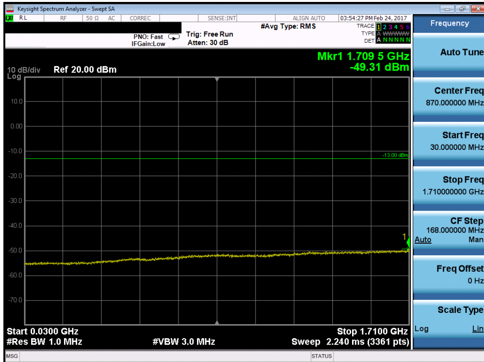
Plot 7-62. Conducted Spurious Plot (Band 4/66 – 20.0MHz QPSK – RB Size 1, RB Offset 0 – Mid Channel)
