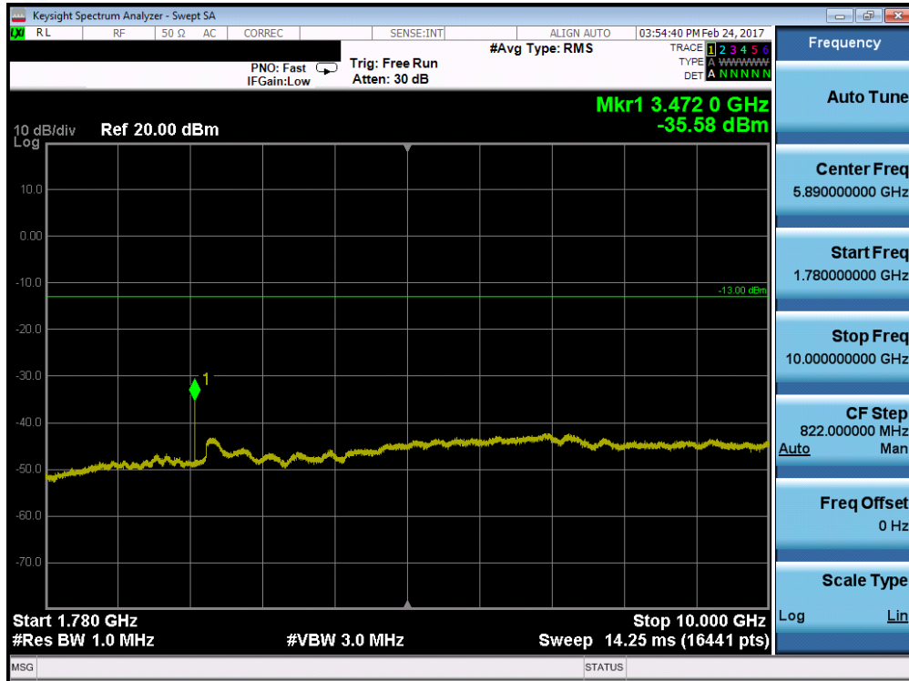
Plot 7-63. Conducted Spurious Plot (Band 4/66 – 20.0MHz QPSK – RB Size 1, RB Offset 0 – Mid Channel)
