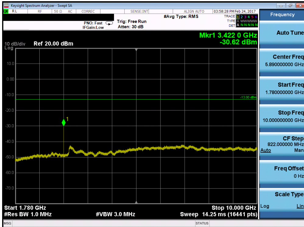
Plot 7-60. Conducted Spurious Plot (Band 4/66 – 20.0MHz QPSK – RB Size 1, RB Offset 0 – Low Channel)
