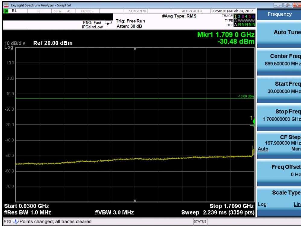
Plot 7-59. Conducted Spurious Plot (Band 4/66 – 20.0MHz QPSK – RB Size 1, RB Offset 0– Low Channel)
