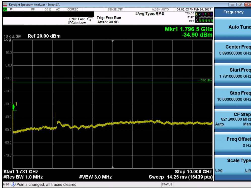
Plot 7-66. Conducted Spurious Plot (Band 4/66 – 20.0MHz QPSK – RB Size 1, RB Offset 0 – High Channel)
