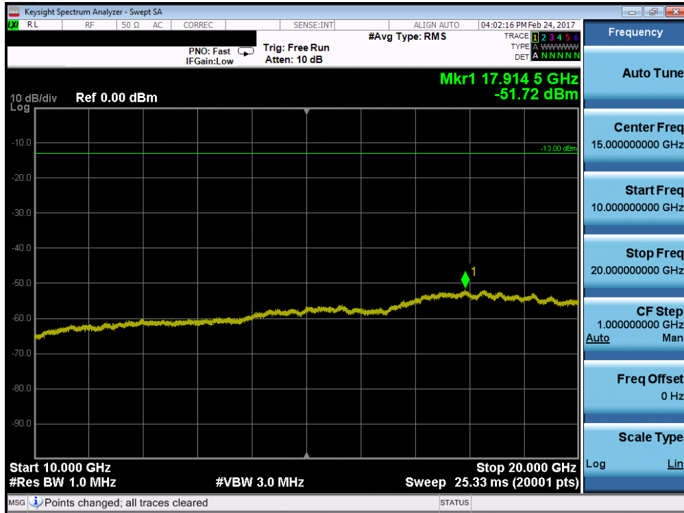
Plot 7-67. Conducted Spurious Plot (Band 4/66 – 20.0MHz QPSK – RB Size 1, RB Offset 0 – High Channel)
