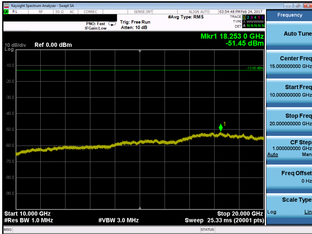
Plot 7-64. Conducted Spurious Plot (Band 4/66 – 20.0MHz QPSK – RB Size 1, RB Offset 0 – Mid Channel)
