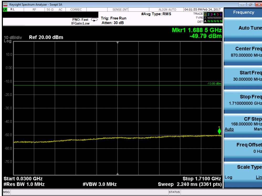
Plot 7-65. Conducted Spurious Plot (Band 4/66 – 20.0MHz QPSK – RB Size 1, RB Offset 0 – High Channel)
