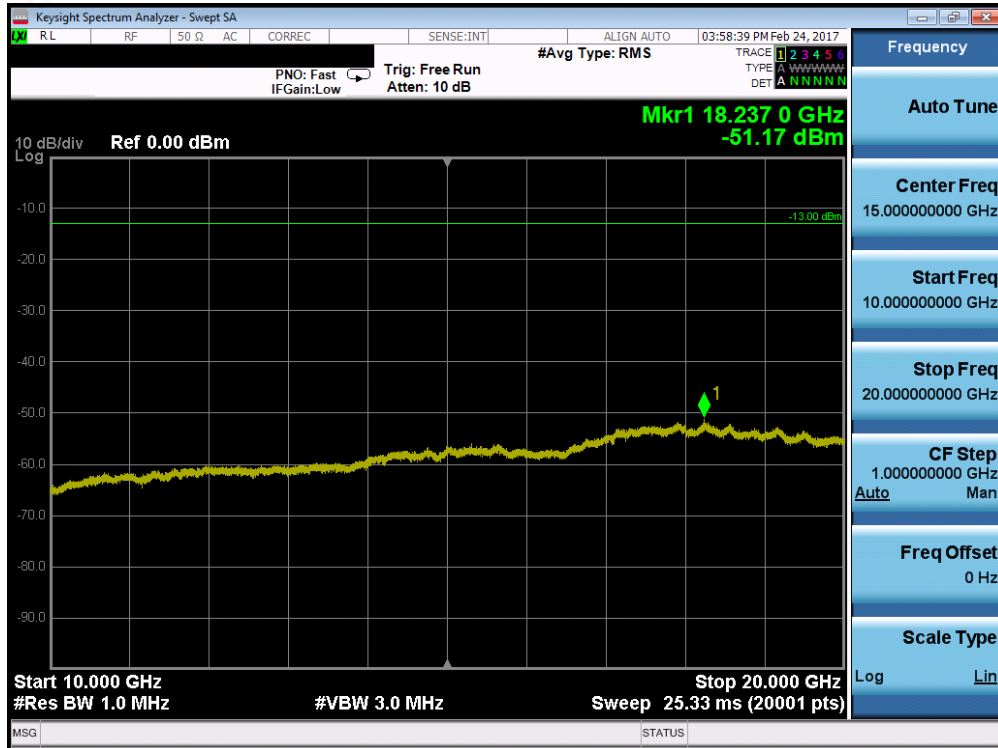
Plot 7-61. Conducted Spurious Plot (Band 4/66 – 20.0MHz QPSK – RB Size 1, RB Offset 0 – Low Channel)
