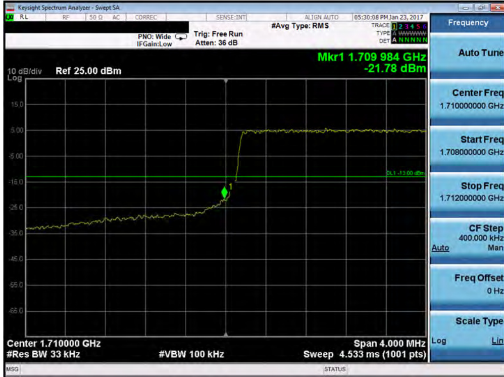
Plot 7-99. Lower Band Edge Plot (Band 4 – 3.0MHz QPSK – RB Size 15)
