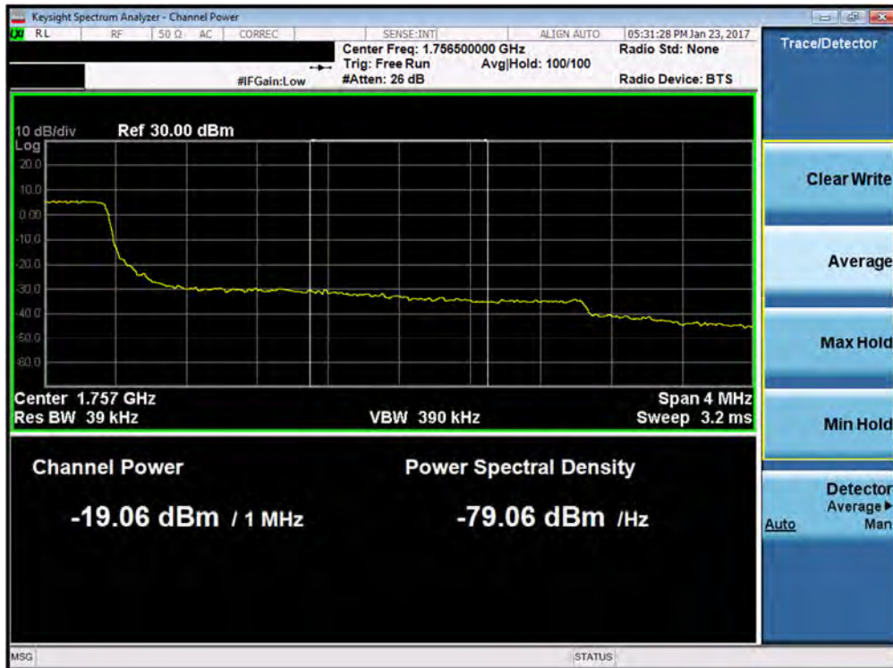
Plot 7-102. Upper Extended Band Edge Plot (Band 4 – 3.0MHz QPSK – RB Size 15)
