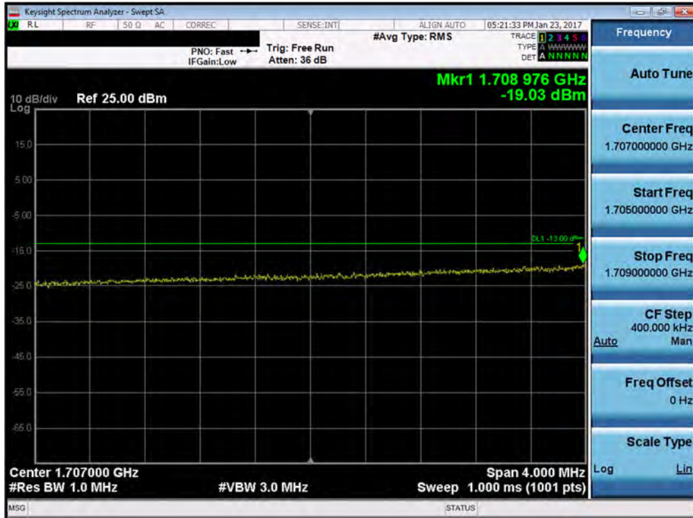
Plot 7-108. Lower Extended Band Edge Plot (Band 4 – 10.0MHz QPSK – RB Size 50)
