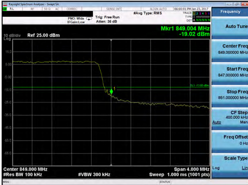
Plot 7-92. Upper Band Edge Plot (Band 5 – 5.0MHz QPSK – RB Size 25)
