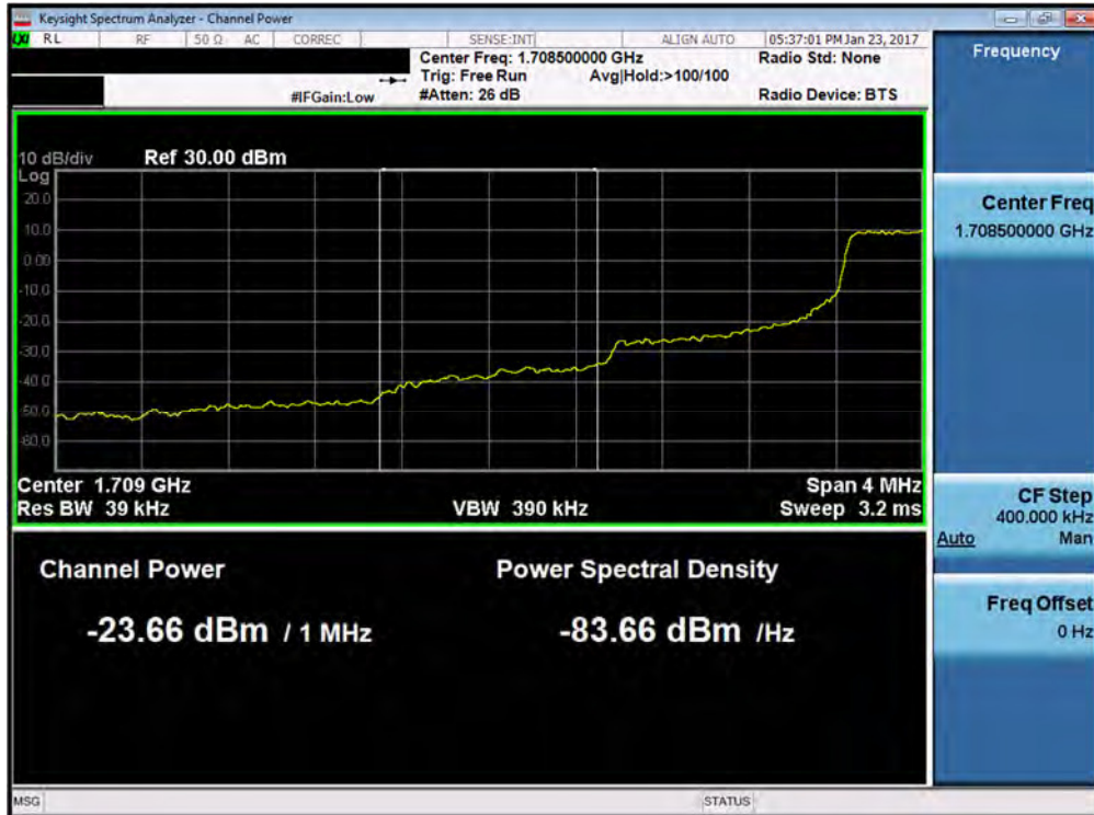
Plot 7-96. Lower Extended Band Edge Plot (Band 4 – 1.4MHz QPSK – RB Size 6)
