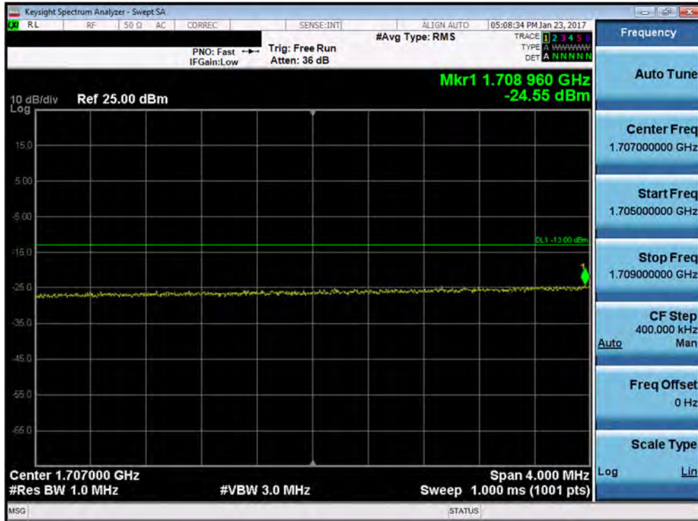
Plot 7-116. Lower Extended Band Edge Plot (Band 4 – 20.0MHz QPSK – RB Size 100)
