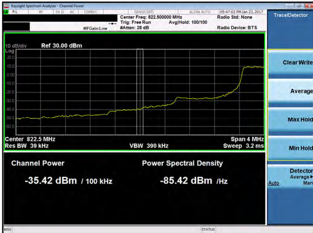
Plot 7-86. Lower Extended Band Edge Plot (Band 5 – 1.4MHz QPSK – RB Size 6)
