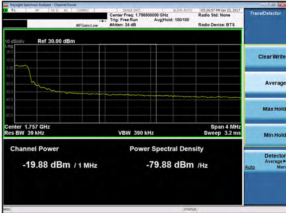
Plot 7-106. Upper Extended Band Edge Plot (Band 4 – 5.0MHz QPSK – RB Size 25)
