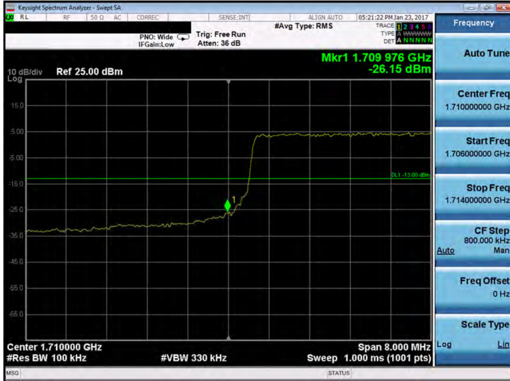
Plot 7-107. Lower Band Edge Plot (Band 4 – 10.0MHz QPSK – RB Size 50)
