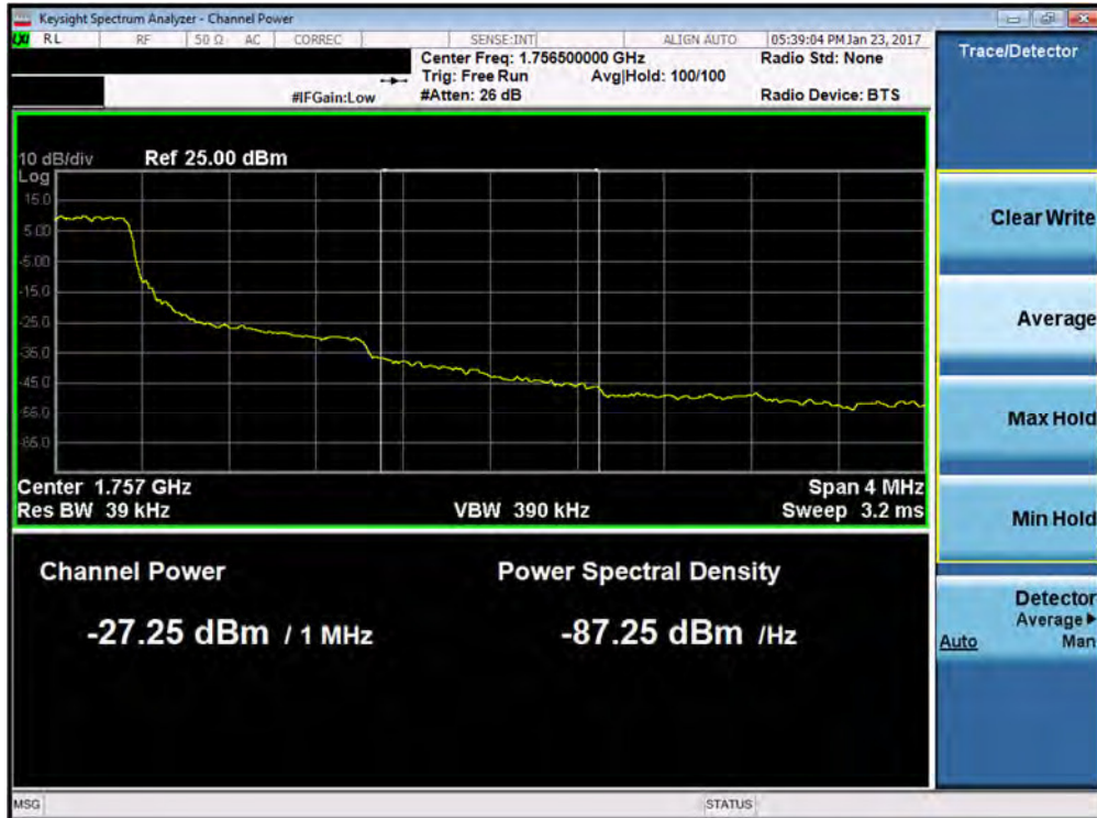
Plot 7-98. Upper Extended Band Edge Plot (Band 4 – 1.4MHz QPSK – RB Size 6)
