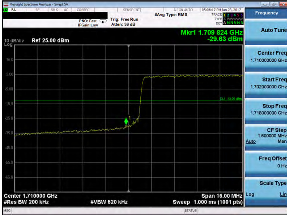
Plot 7-115. Lower Band Edge Plot (Band 4 – 20.0MHz QPSK – RB Size 100)
