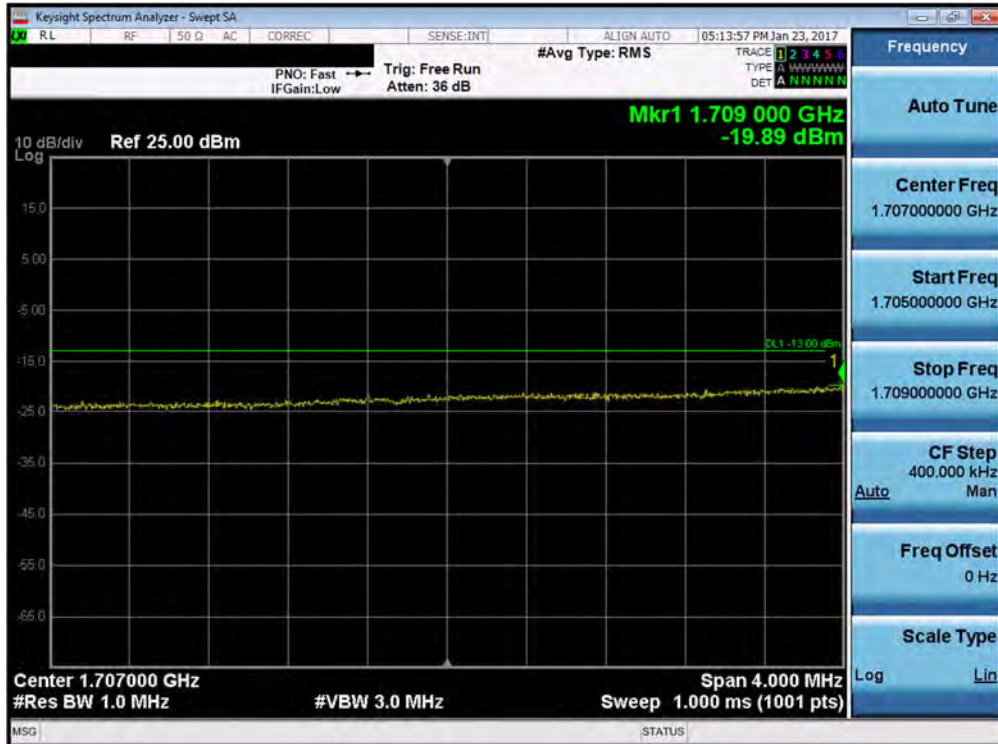
Plot 7-112. Lower Extended Band Edge Plot (Band 4 – 15.0MHz QPSK – RB Size 75)
