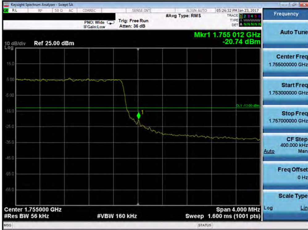
Plot 7-105. Upper Band Edge Plot (Band 4 – 5.0MHz QPSK – RB Size 25)
