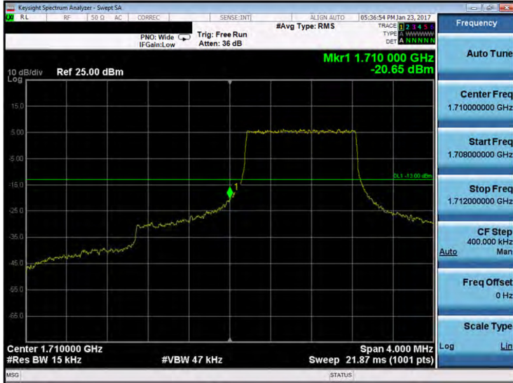
Plot 7-95. Lower Band Edge Plot (Band 4 – 1.4MHz QPSK – RB Size 6)
