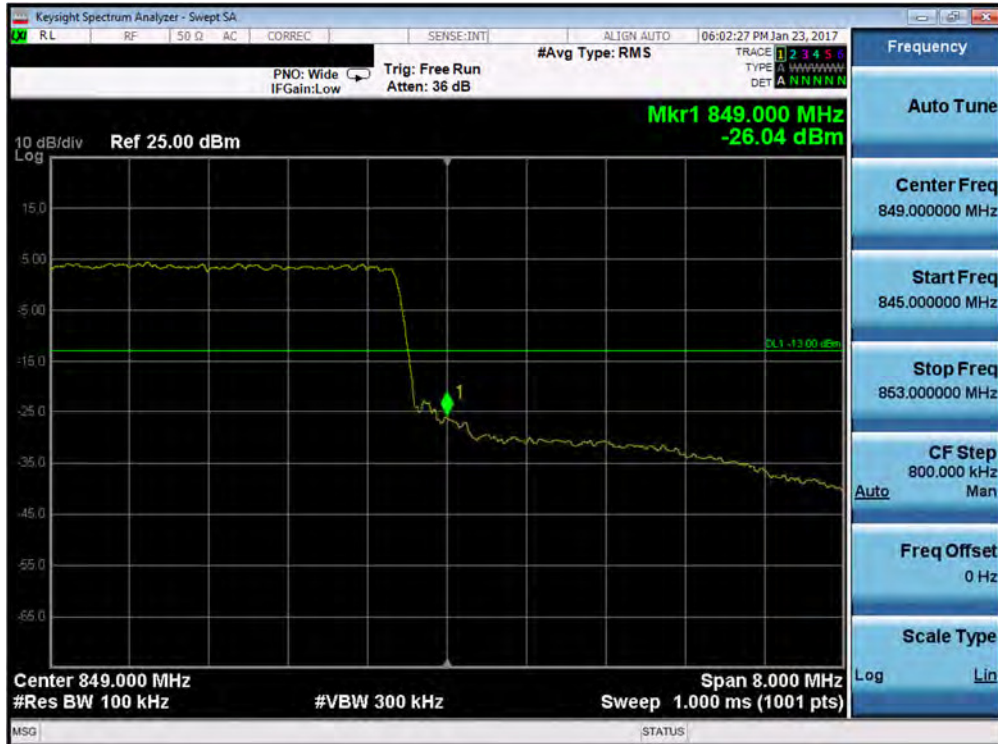
Plot 7-94. Upper Band Edge Plot (Band 5 – 10.0MHz QPSK – RB Size 50)
