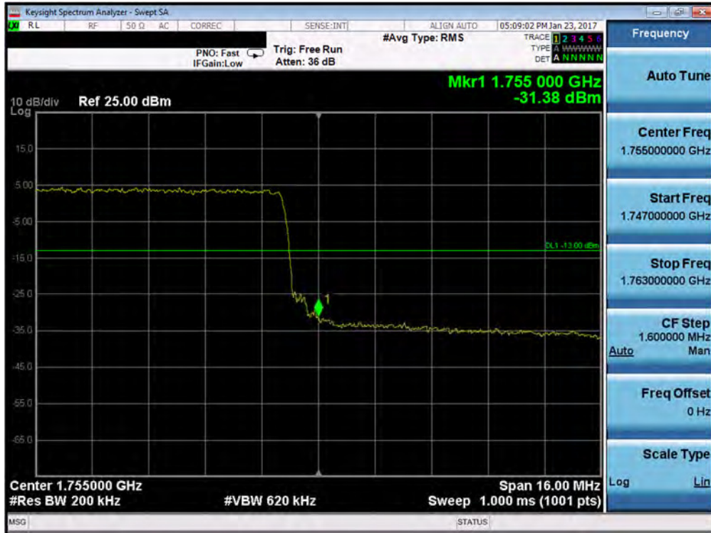
Plot 7-117. Upper Band Edge Plot (Band 4 – 20.0MHz QPSK – RB Size 100)
