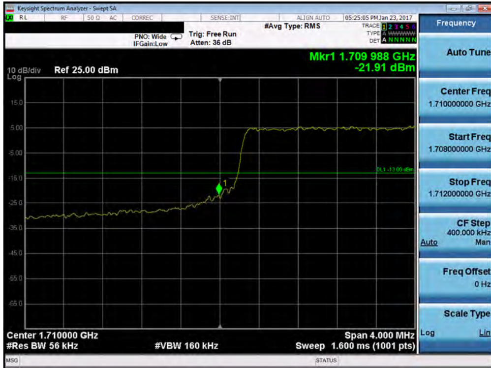
Plot 7-103. Lower Band Edge Plot (Band 4 – 5.0MHz QPSK – RB Size 25)
