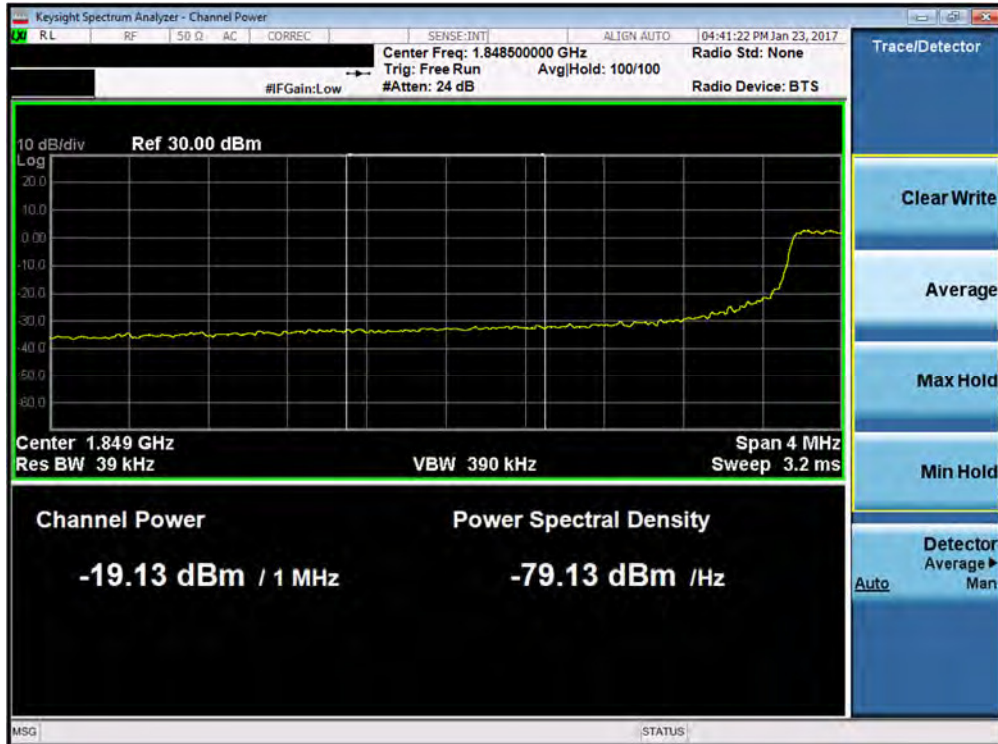
Plot 7-128. Lower Extended Band Edge Plot (Band 2 – 5.0MHz QPSK – RB Size 25)
