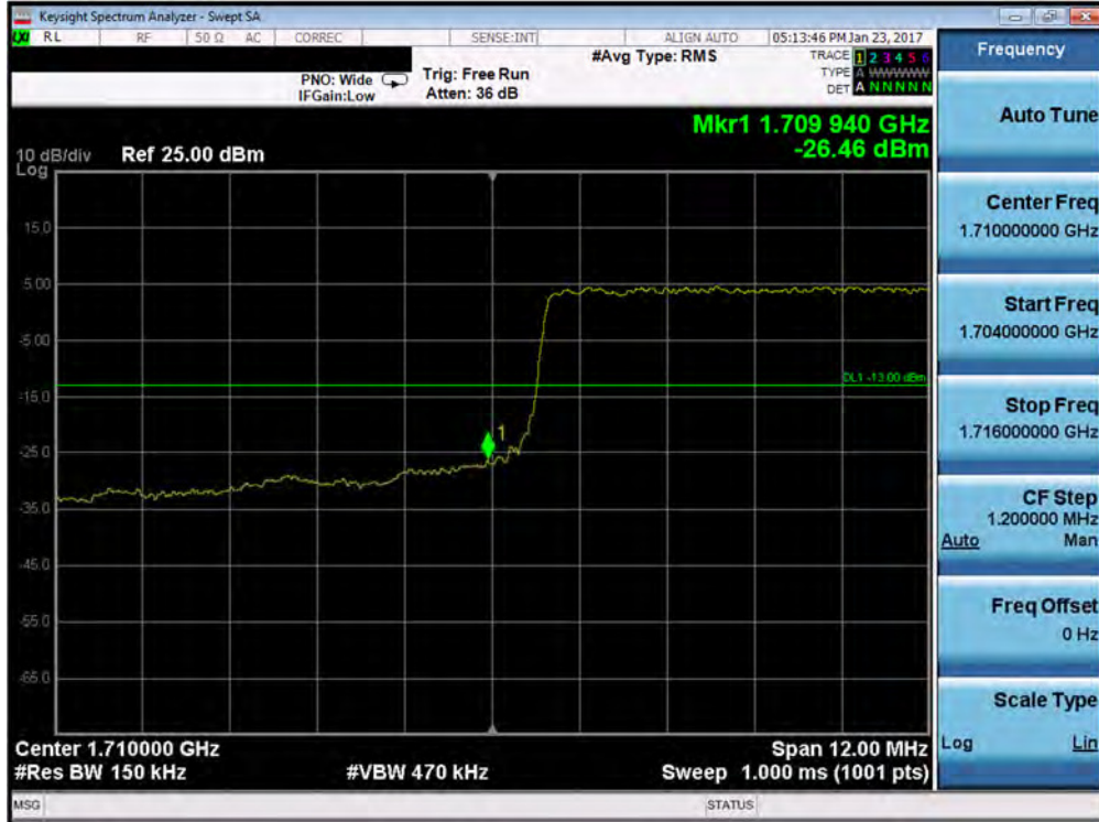
Plot 7-111. Lower Band Edge Plot (Band 4 – 15.0MHz QPSK – RB Size 75)
