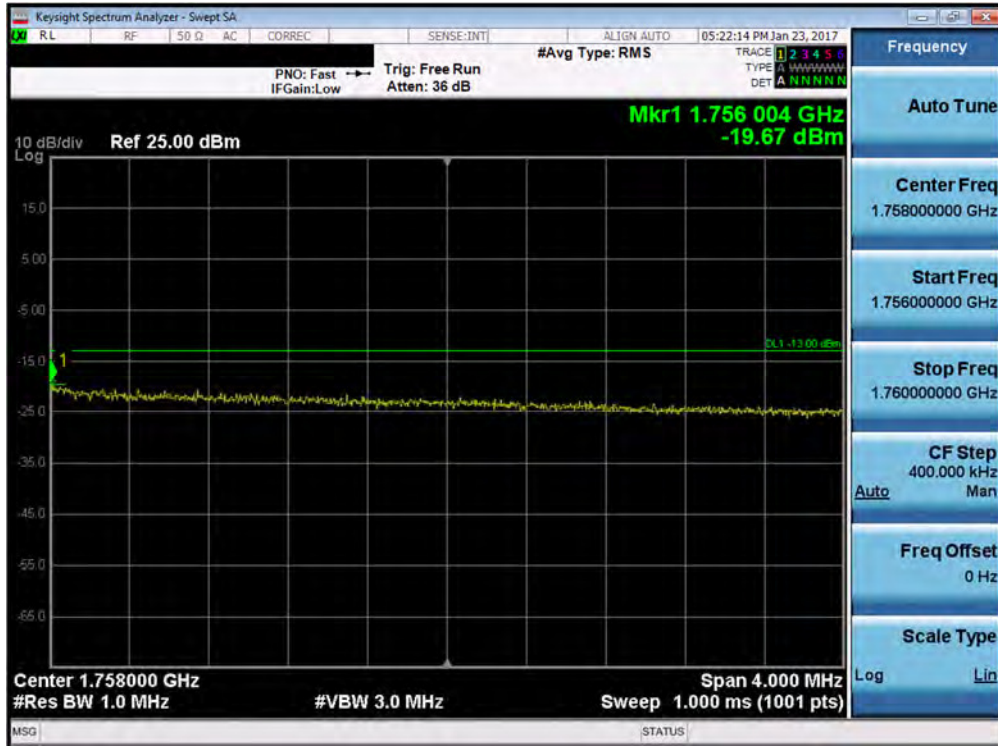
Plot 7-110. Upper Extended Band Edge Plot (Band 4 – 10.0MHz QPSK – RB Size 50)
