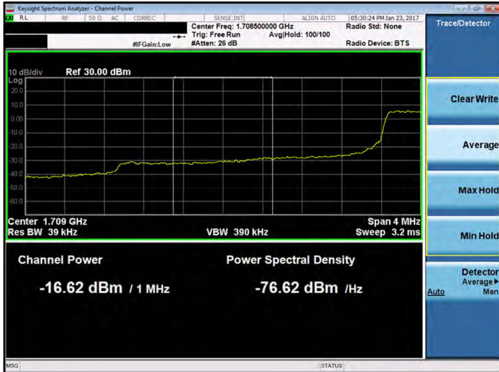
Plot 7-100. Lower Extended Band Edge Plot (Band 4 – 3.0MHz QPSK – RB Size 15)
