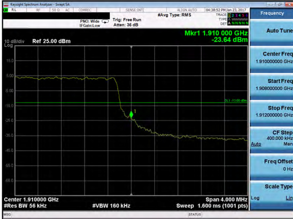
Plot 7-129. Upper Band Edge Plot (Band 2 – 5.0MHz QPSK – RB Size 25)
