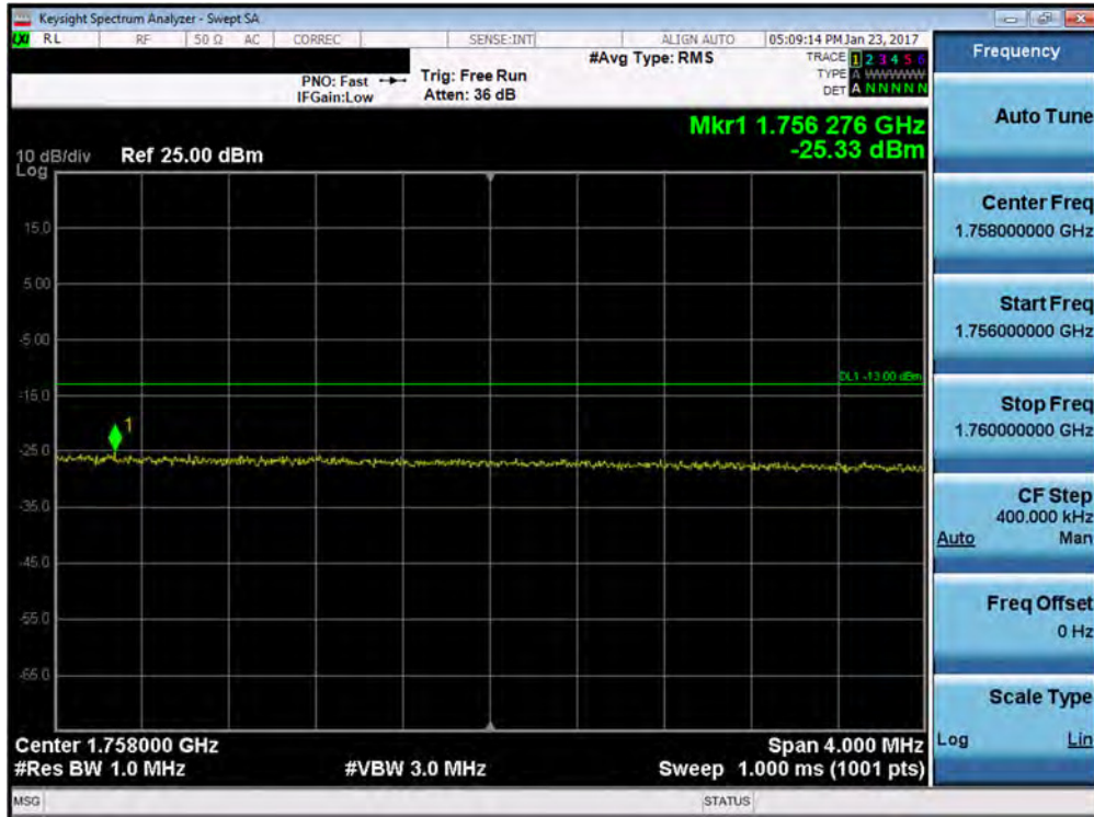
Plot 7-118. Upper Extended Band Edge Plot (Band 4 – 20.0MHz QPSK – RB Size 100)
