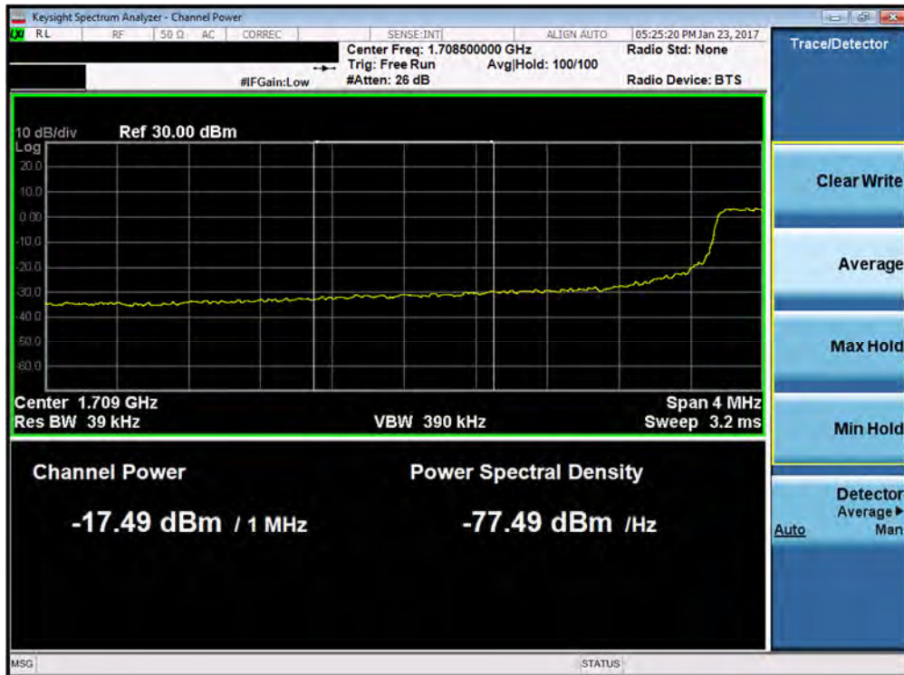
Plot 7-104. Lower Extended Band Edge Plot (Band 4 – 5.0MHz QPSK – RB Size 25)
