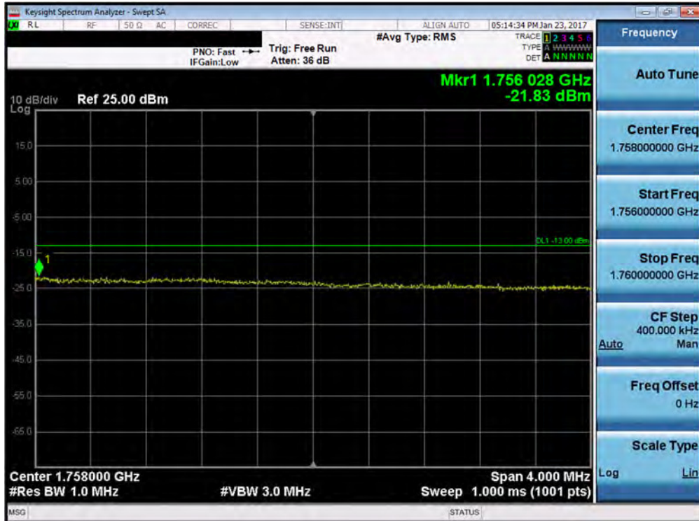
Plot 7-114. Upper Extended Band Edge Plot (Band 4 – 15.0MHz QPSK – RB Size 75)
