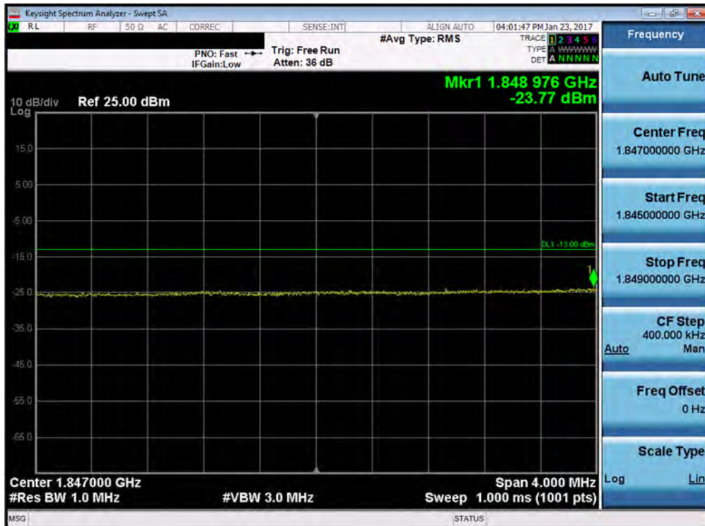
Plot 7-140. Lower Extended Band Edge Plot (Band 2 – 20.0MHz QPSK – RB Size 100)
