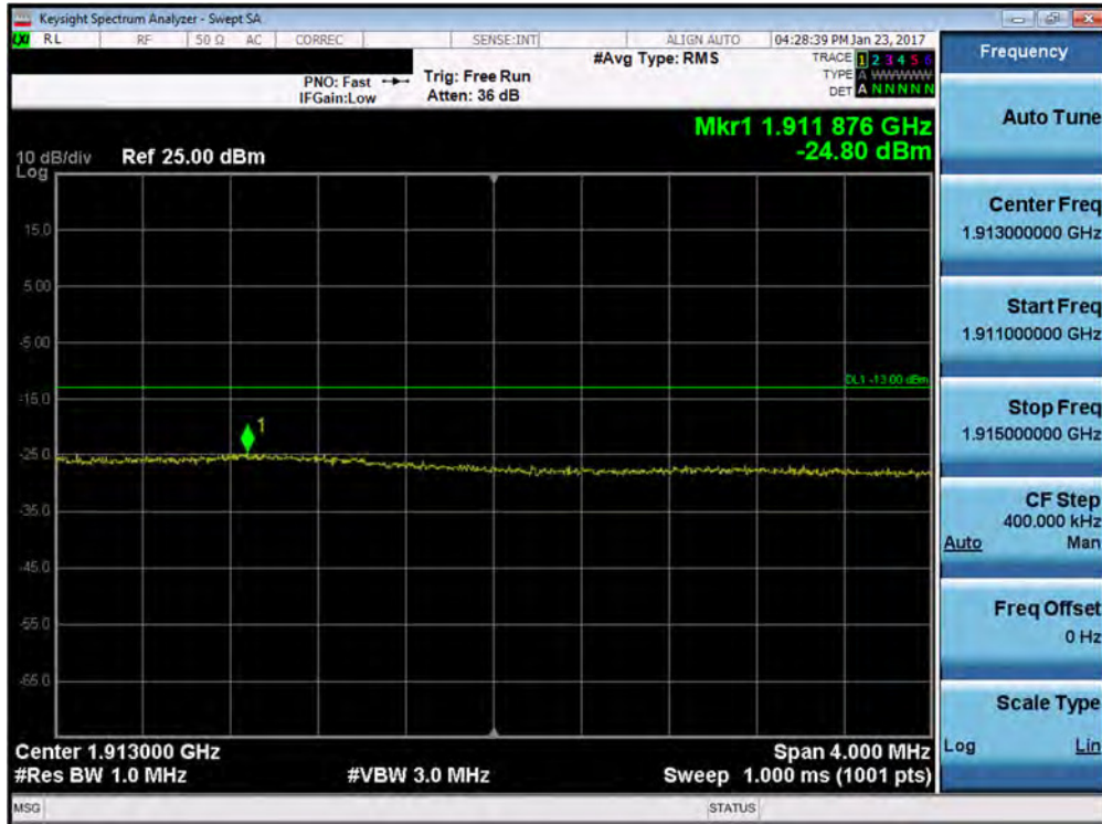
Plot 7-138. Upper Extended Band Edge Plot (Band 2 – 15.0MHz QPSK – RB Size 75)
