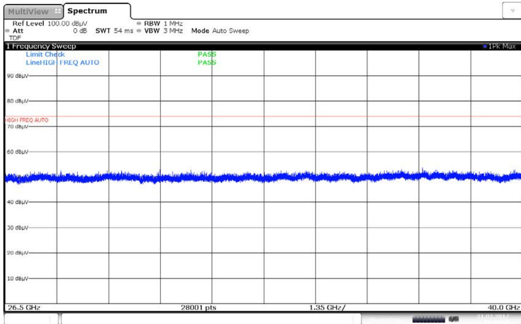
Plot 7-90. Radiated Spurious Plot above 26.5GHz - 40GHz (802.11a – Ant. Pol. V)
