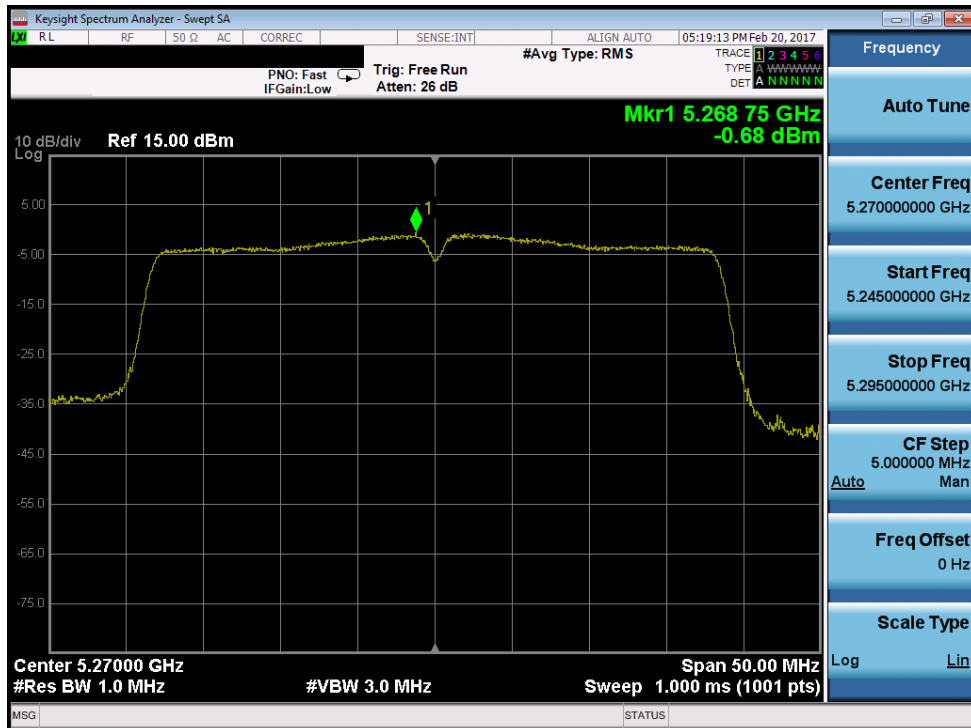
Plot 7-55. Power Spectral Density Plot (40MHz BW 802.11a/n (UNII Band 2A) – Ch. 54)
