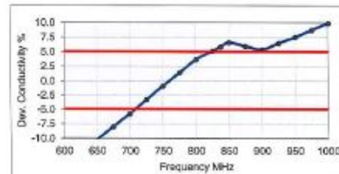
Figure D-2 750 MHz Head Tissue Equivalent Matter
