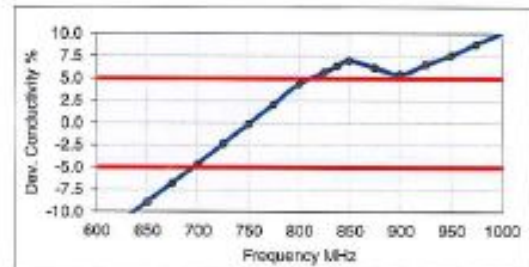
Figure D-3 750 MHz Body Tissue Equivalent Matter
