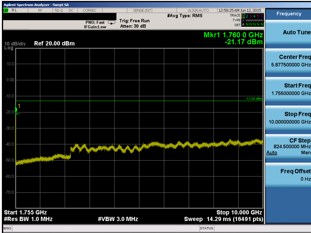
Plot 6-59. Conducted Spurious Plot (Band 4 – 20.0MHz QPSK – RB Size 1, RB Offset 0 – Mid Channel)
