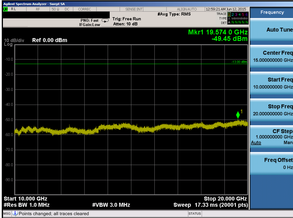
Plot 6-57. Conducted Spurious Plot (Band 4 – 20.0MHz QPSK – RB Size 1, RB Offset 0 – Low Channel)
