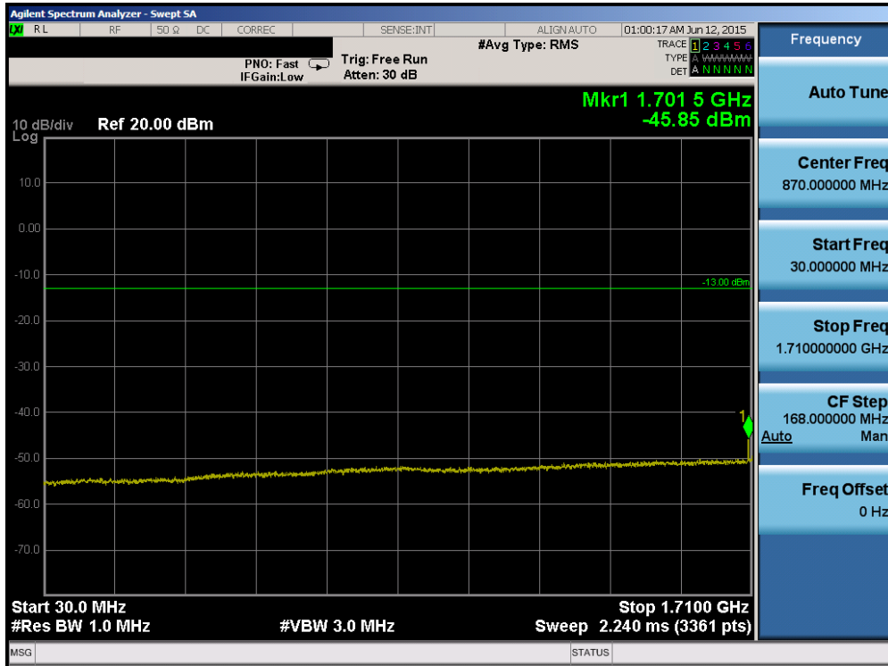
Plot 6-61. Conducted Spurious Plot (Band 4 – 20.0MHz QPSK – RB Size 1, RB Offset 0 – High Channel)
