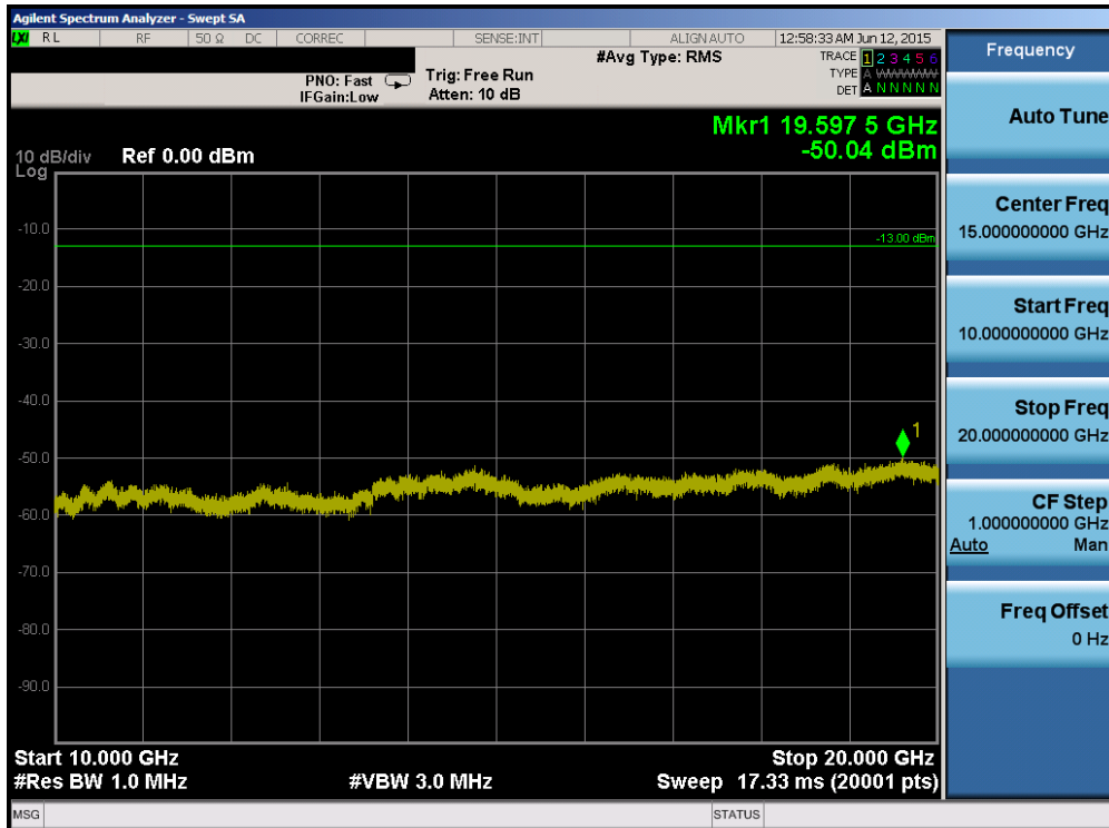
Plot 6-60. Conducted Spurious Plot (Band 4 – 20.0MHz QPSK – RB Size 1, RB Offset 0 – Mid Channel)
