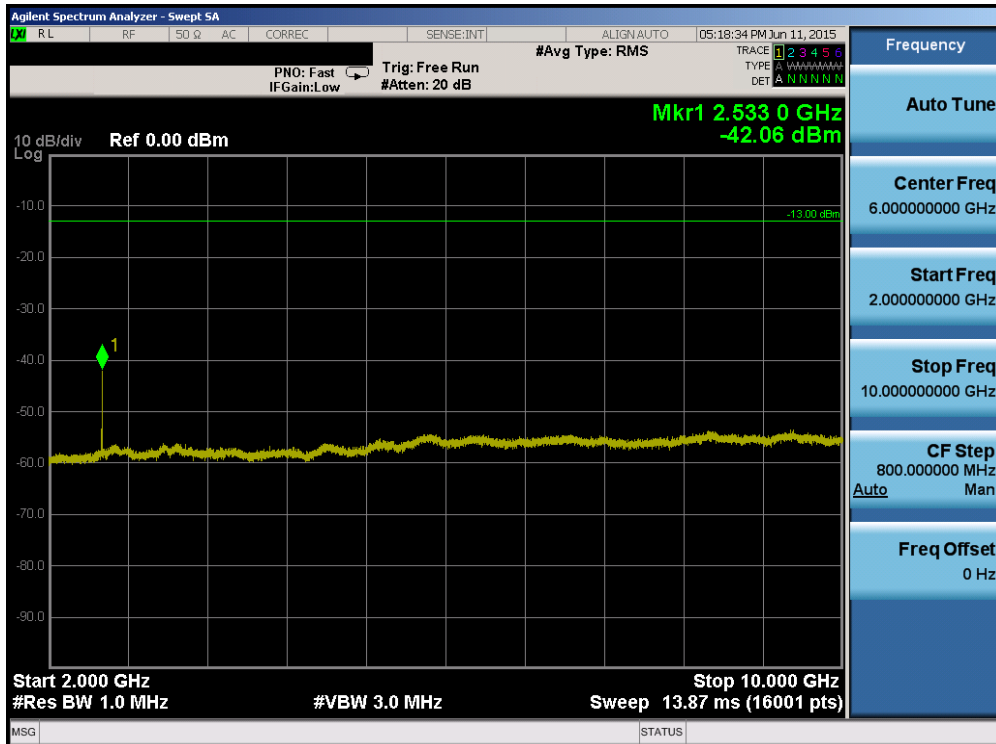
Plot 6-54. Conducted Spurious Plot (Band 5 – 5.0MHz QPSK – RB Size 1, RB Offset 0 – High Channel)
