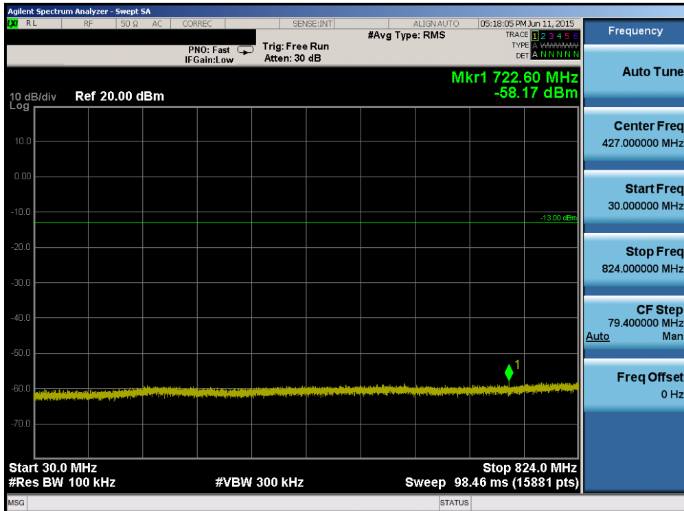
Plot 6-52. Conducted Spurious Plot (Band 5 – 5.0MHz QPSK – RB Size 1, RB Offset 0 – High Channel)
