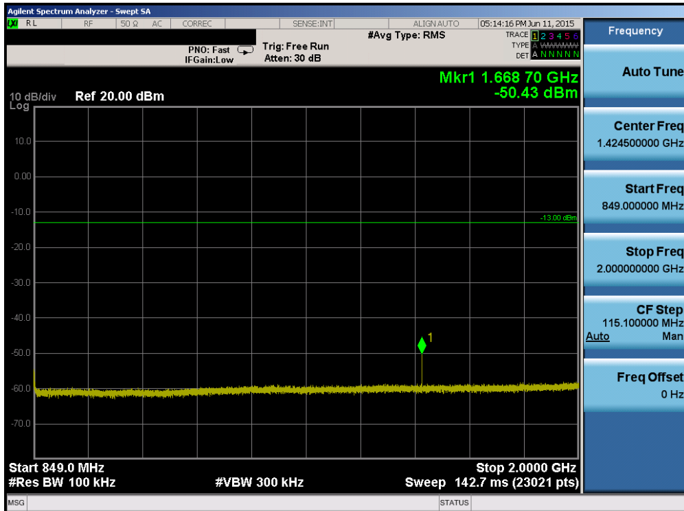
Plot 6-50. Conducted Spurious Plot (Band 5 – 5.0MHz QPSK – RB Size 1, RB Offset 0 – Mid Channel)
