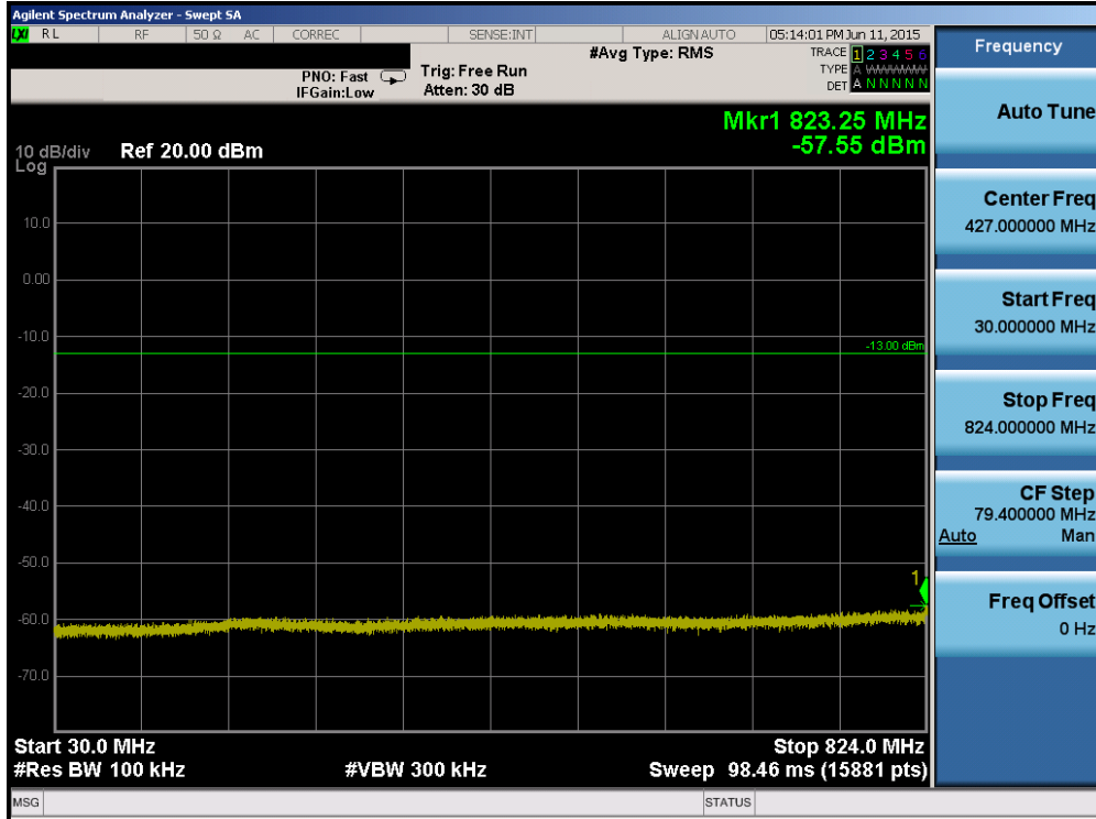
Plot 6-49. Conducted Spurious Plot (Band 5 – 5.0MHz QPSK – RB Size 1, RB Offset 0 – Mid Channel)
