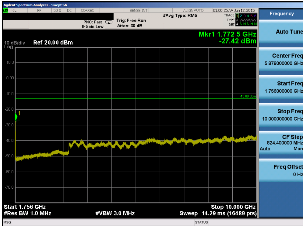
Plot 6-62. Conducted Spurious Plot (Band 4 – 20.0MHz QPSK – RB Size 1, RB Offset 0 – High Channel)
