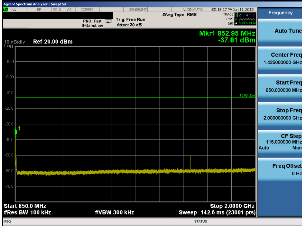
Plot 6-53. Conducted Spurious Plot (Band 5 – 5.0MHz QPSK – RB Size 1, RB Offset 0 – High Channel)
