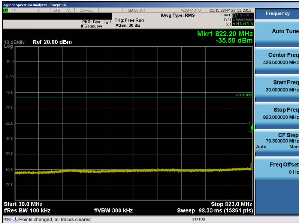
Plot 6-46. Conducted Spurious Plot (Band 5 – 5.0MHz QPSK – RB Size 1, RB Offset 0 – Low Channel)
