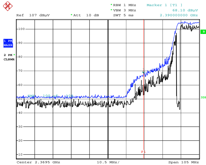
Radiated Restricted Band Edges plot – Peak Reading (802.11g Ch.2)
