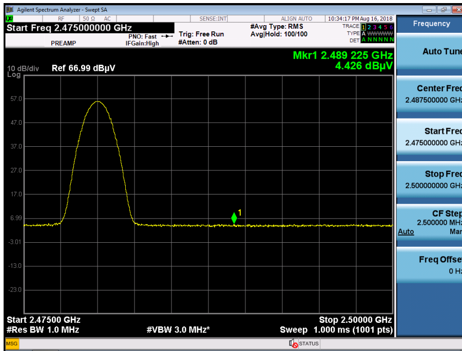
Radiated Restricted Band Edges plot – Average Reading (Ch.19)
