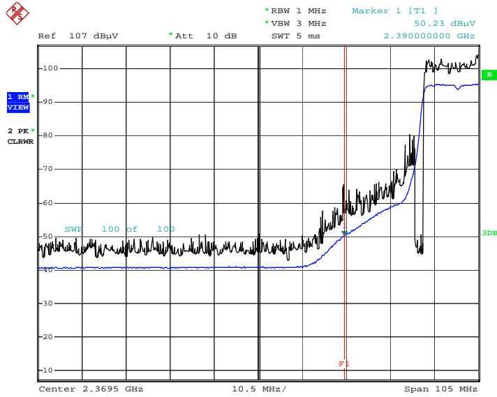
Radiated Restricted Band Edges plot – Average Reading (802.11g Ch.2)
