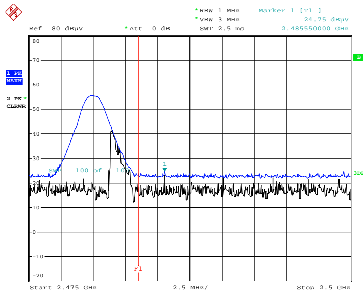
Radiated Band Edges plot – Peak Reading (Ch.78)
