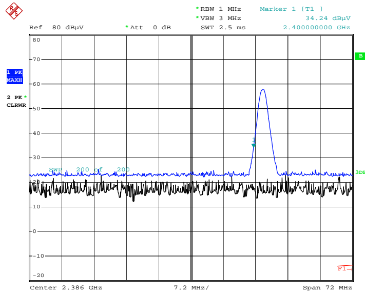
Radiated Band Edges plot – Peak Reading (Ch.0)
