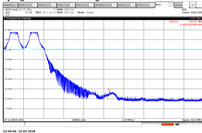
[GFSK Hopping Mode] High Channel BandEdge
