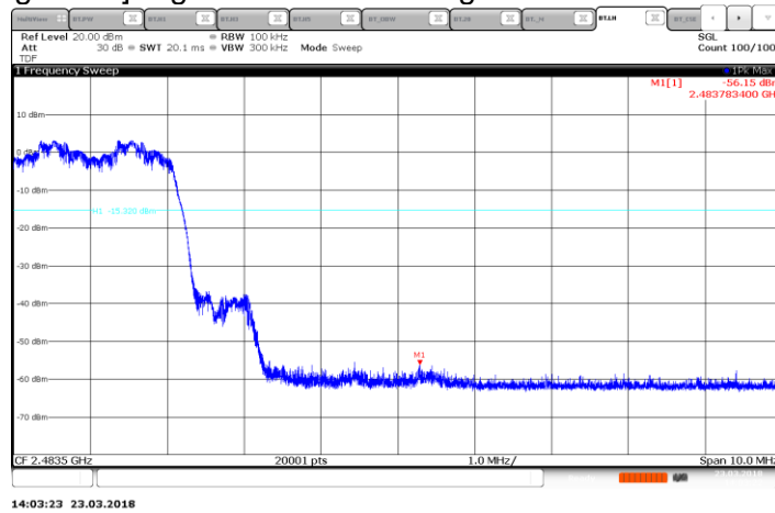
[PI/4-DQPSK Hopping Mode] High Channel BandEdge
