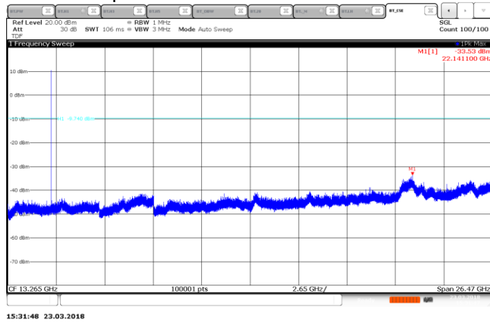
[GFSK] Low Channel Spurious
