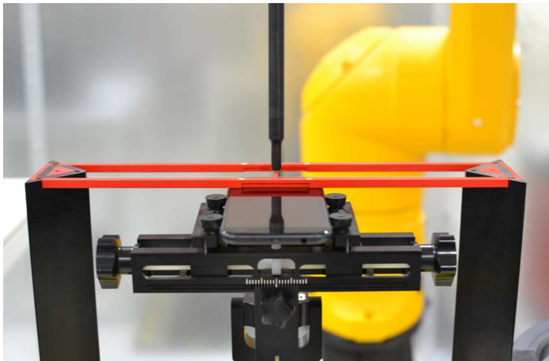
Figure 18-1 Ear Reference Point HAC Phantom Alignment
