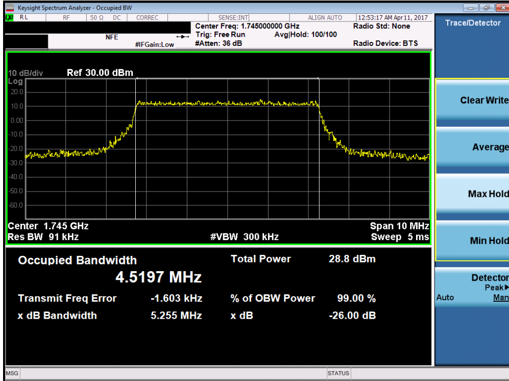
Plot 7-21. Occupied Bandwidth Plot (Band 4/66 – 5.0MHz QPSK – RB Size 25)
