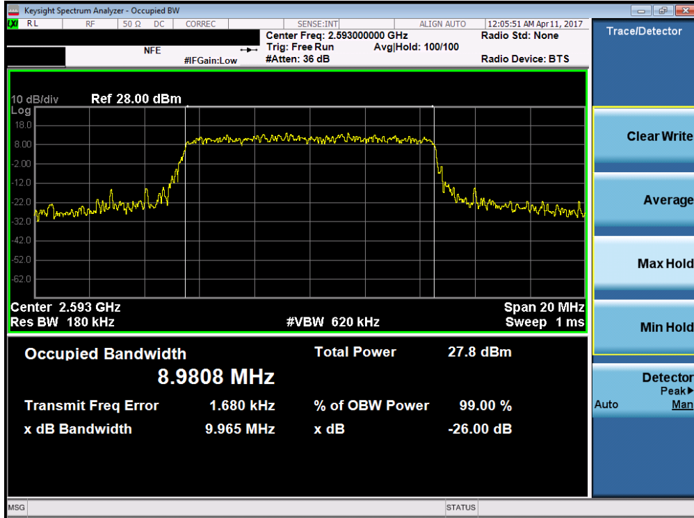
Plot 7-43. Occupied Bandwidth Plot (Band 41 – 10.0MHz QPSK – RB Size 50)
