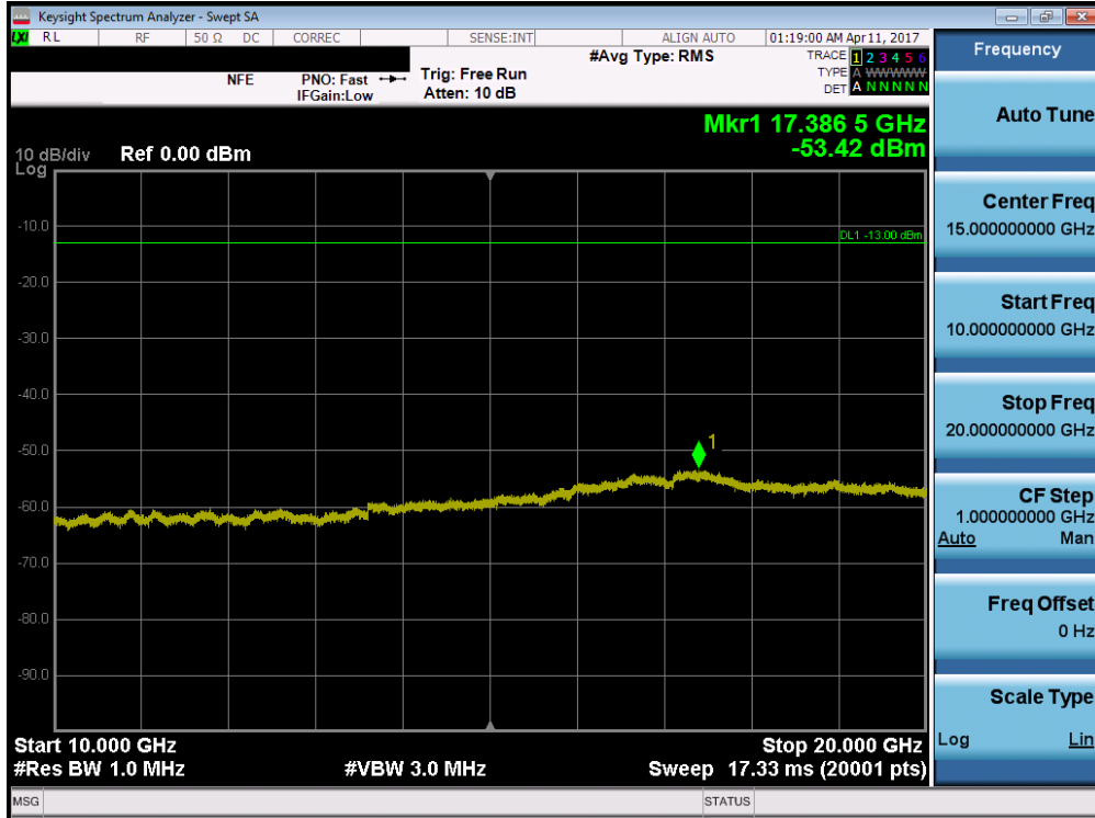
Plot 7-75. Conducted Spurious Plot (Band 4/66 – 10.0MHz QPSK – RB Size 1, RB Offset 0 – High Channel)
