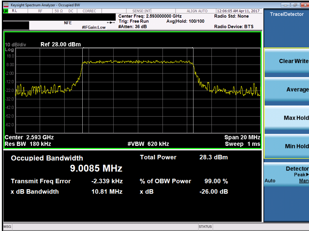
Plot 7-44. Occupied Bandwidth Plot (Band 41 – 10.0MHz 16-QAM – RB Size 50)
