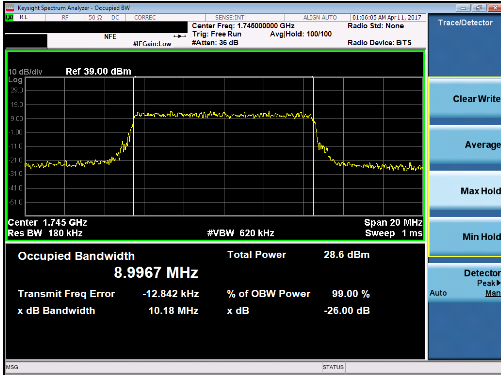
Plot 7-23. Occupied Bandwidth Plot (Band 4/66 – 10.0MHz QPSK – RB Size 50)
