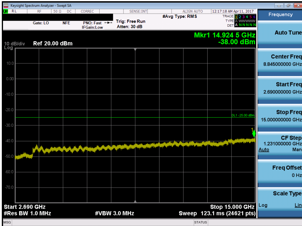
Plot 7-86. Conducted Spurious Plot (Band 41 – 15.0MHz QPSK – RB Size 1, RB Offset 0 – Low Channel)
