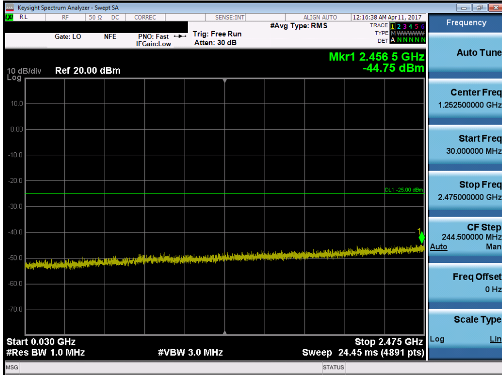
Plot 7-85. Conducted Spurious Plot (Band 41 – 15.0MHz QPSK – RB Size 1, RB Offset 0 – Low Channel)
