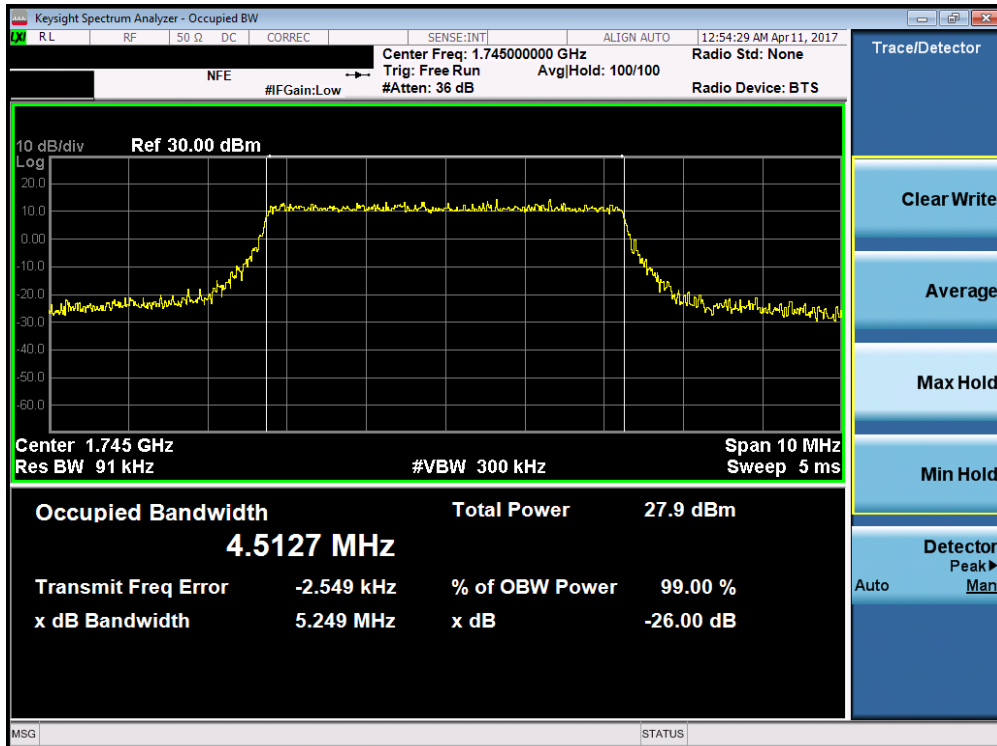
Plot 7-22. Occupied Bandwidth Plot (Band 4/66 – 5.0MHz 16-QAM – RB Size 25)
