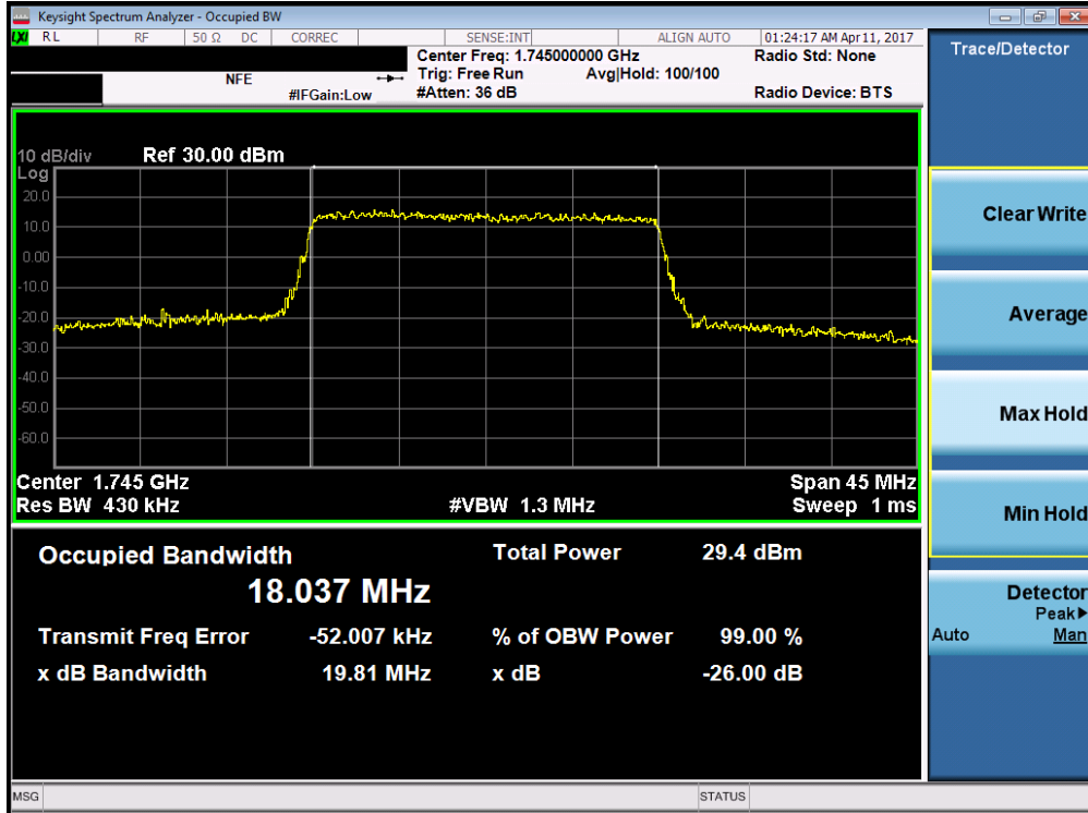
Plot 7-27. Occupied Bandwidth Plot (Band 4/66 – 20.0MHz QPSK – RB Size 100)
