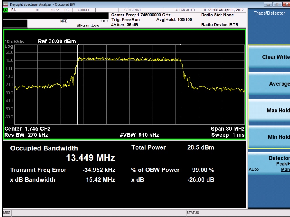
Plot 7-25. Occupied Bandwidth Plot (Band 4/66 – 15.0MHz QPSK – RB Size 75)
