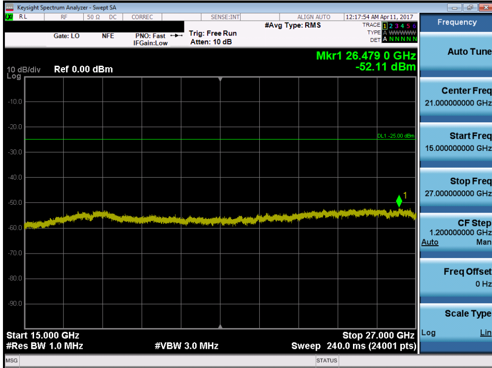
Plot 7-87. Conducted Spurious Plot (Band 41 – 15.0MHz QPSK – RB Size 1, RB Offset 0 – Low Channel)
