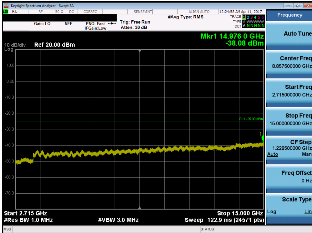
Plot 7-92. Conducted Spurious Plot (Band 41 – 15.0MHz QPSK – RB Size 1, RB Offset 0 – High Channel)
