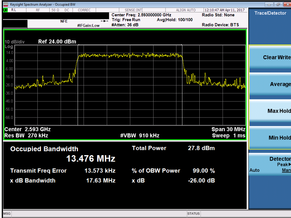
Plot 7-45. Occupied Bandwidth Plot (Band 41 – 15.0MHz QPSK – RB Size 75)
