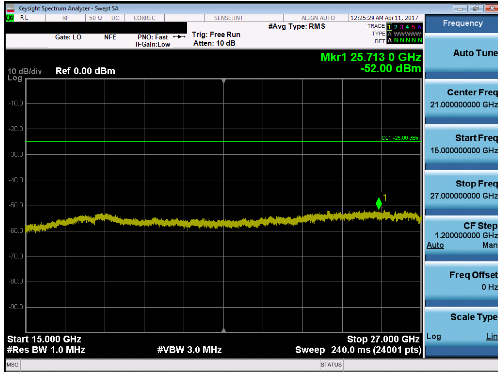
Plot 7-93. Conducted Spurious Plot (Band 41 – 15.0MHz QPSK – RB Size 1, RB Offset 0 – High Channel)
