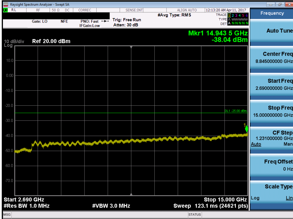
Plot 7-89. Conducted Spurious Plot (Band 41 – 15.0MHz QPSK – RB Size 1, RB Offset 0 – Mid Channel)
