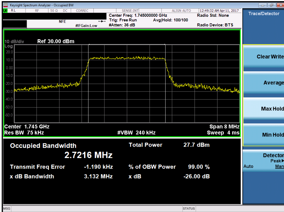
Plot 7-20. Occupied Bandwidth Plot (Band 4/66 – 3.0MHz 16-QAM – RB Size 15)
