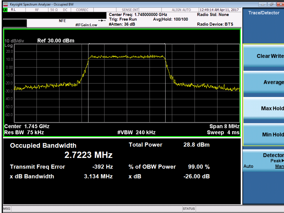
Plot 7-19. Occupied Bandwidth Plot (Band 4/66 – 3.0MHz QPSK – RB Size 15)
