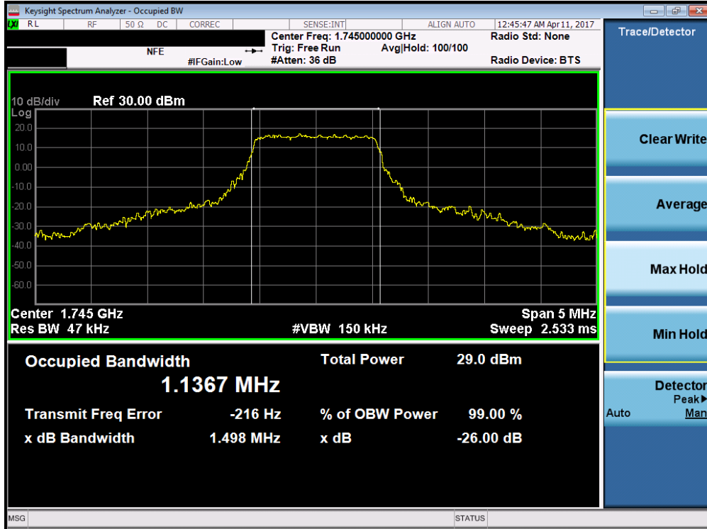
Plot 7-17. Occupied Bandwidth Plot (Band 4/66 – 1.4MHz QPSK – RB Size 6)
