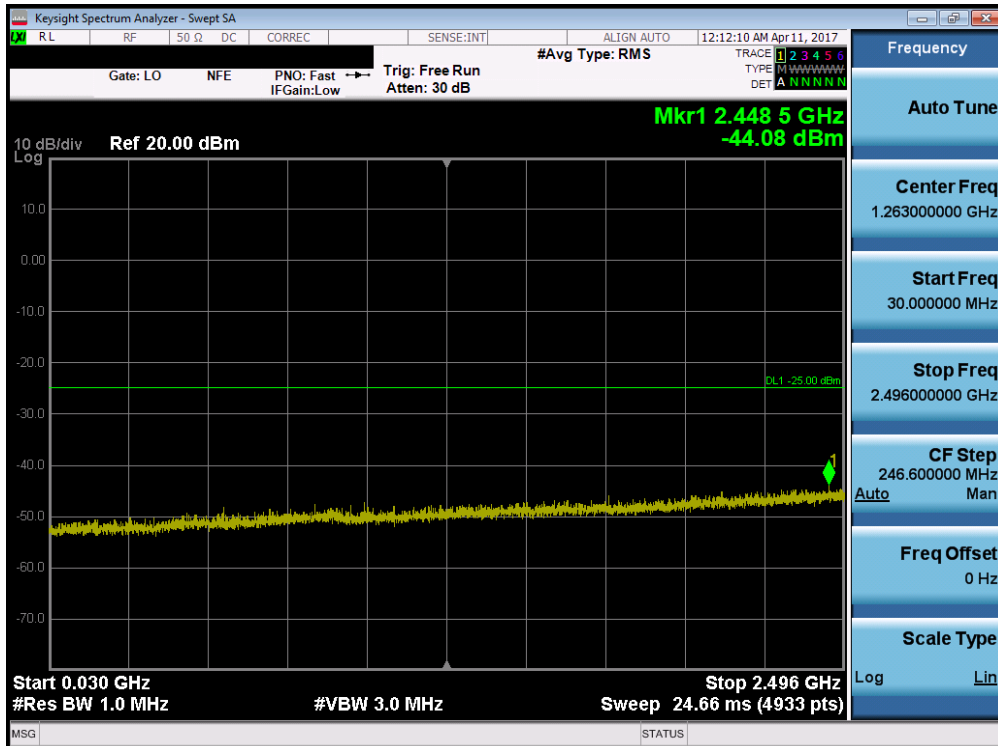
Plot 7-88. Conducted Spurious Plot (Band 41 – 15.0MHz QPSK – RB Size 1, RB Offset 0 – Mid Channel)
