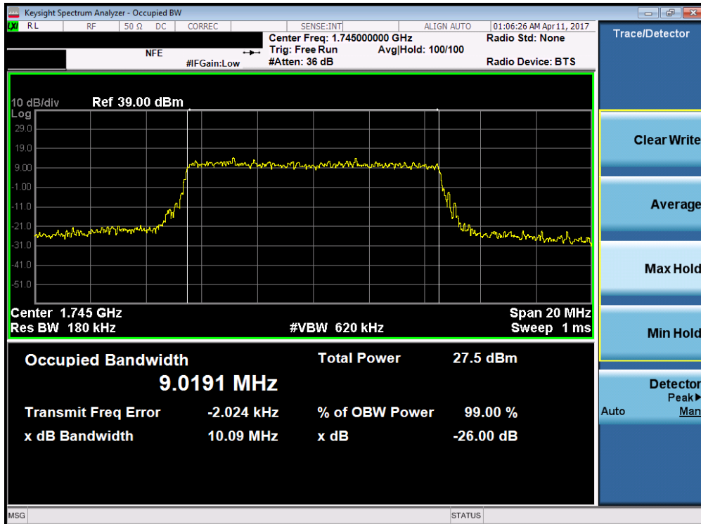
Plot 7-24. Occupied Bandwidth Plot (Band 4/66 – 10.0MHz 16-QAM – RB Size 50)
