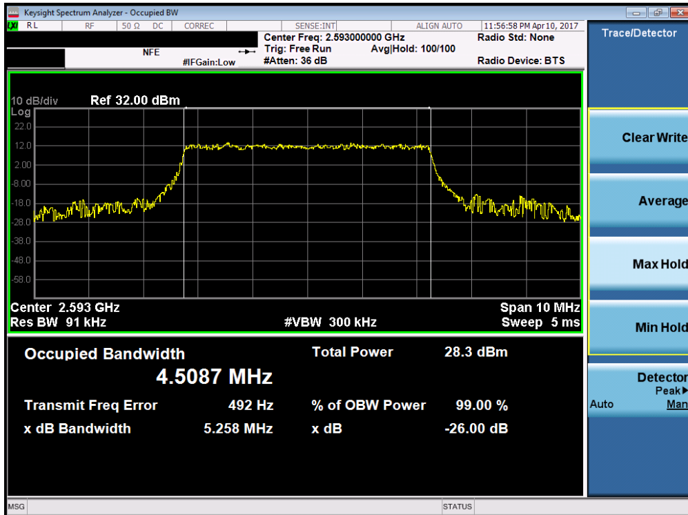
Plot 7-42. Occupied Bandwidth Plot (Band 41 – 5.0MHz 16-QAM – RB Size 25)
