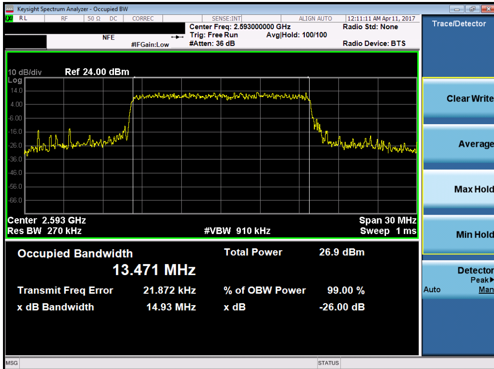
Plot 7-46. Occupied Bandwidth Plot (Band 41 – 15.0MHz 16-QAM – RB Size 75)
