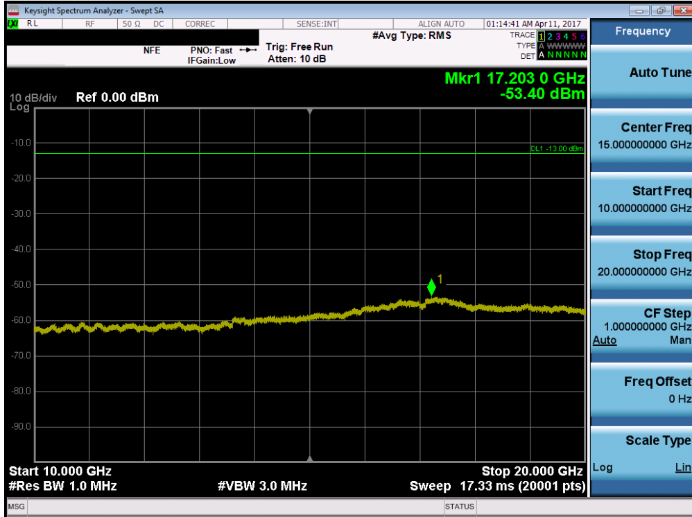
Plot 7-69. Conducted Spurious Plot (Band 4/66 – 10.0MHz QPSK – RB Size 1, RB Offset 0 – Low Channel)
