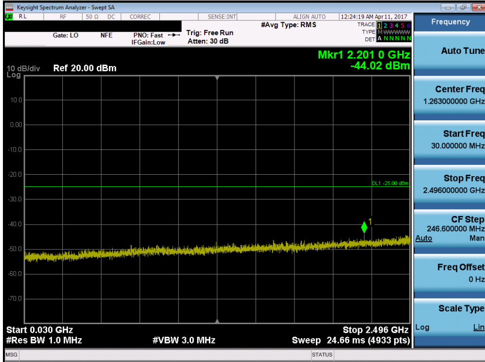
Plot 7-91. Conducted Spurious Plot (Band 41 – 15.0MHz QPSK – RB Size 1, RB Offset 0 – High Channel)
