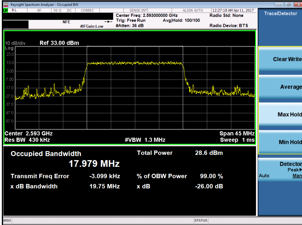
Plot 7-47. Occupied Bandwidth Plot (Band 41 – 20.0MHz QPSK – RB Size 100)
