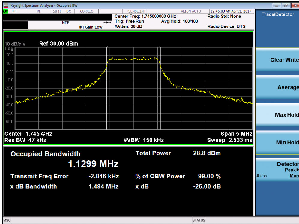
Plot 7-18. Occupied Bandwidth Plot (Band 4/66 – 1.4MHz 16-QAM – RB Size 6)
