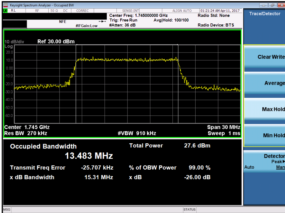
Plot 7-26. Occupied Bandwidth Plot (Band 4/66 – 15.0MHz 16-QAM – RB Size 75)
