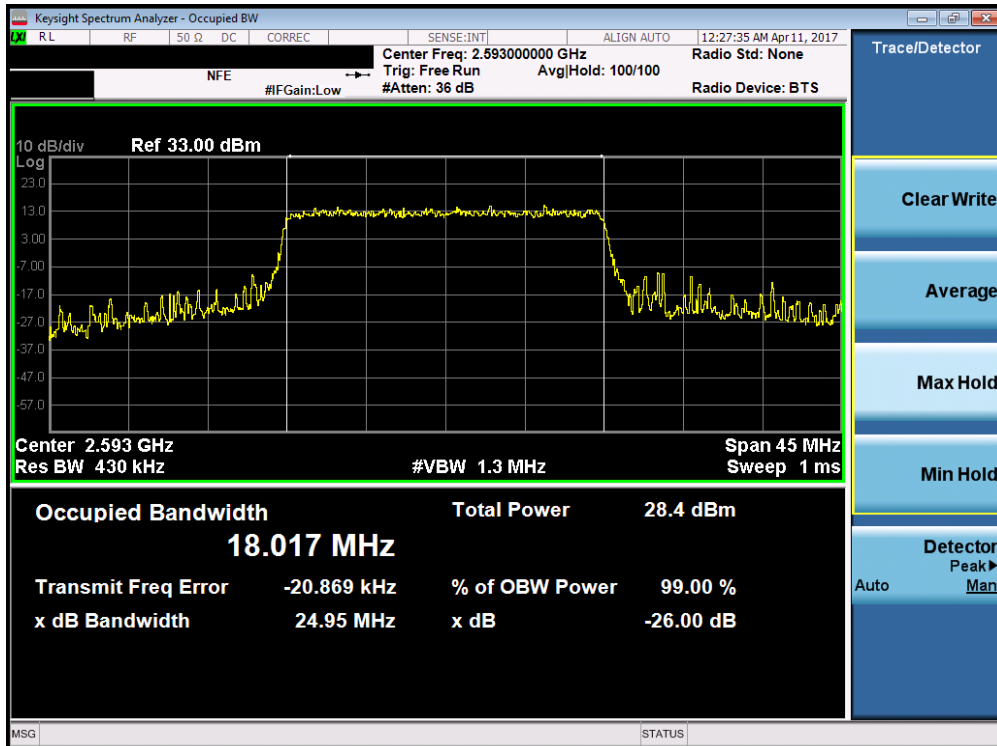
Plot 7-48. Occupied Bandwidth Plot (Band 41 – 20.0MHz 16-QAM – RB Size 100)
