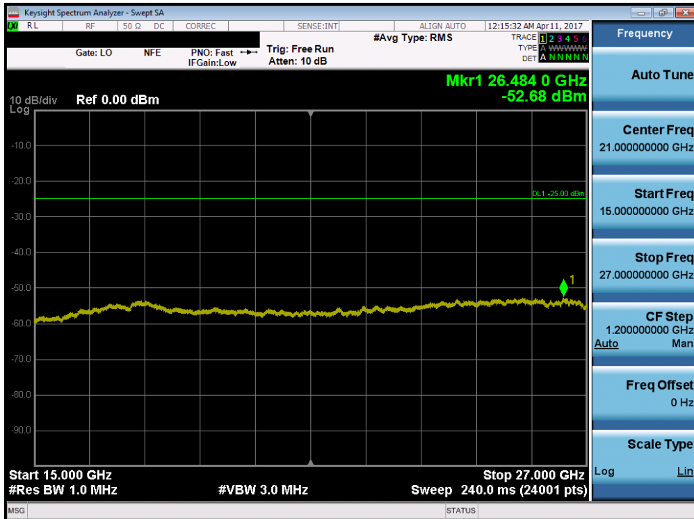
Plot 7-90. Conducted Spurious Plot (Band 41 – 15.0MHz QPSK – RB Size 1, RB Offset 0 – Mid Channel)
