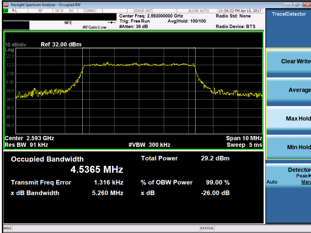
Plot 7-41. Occupied Bandwidth Plot (Band 41 – 5.0MHz QPSK – RB Size 25)
