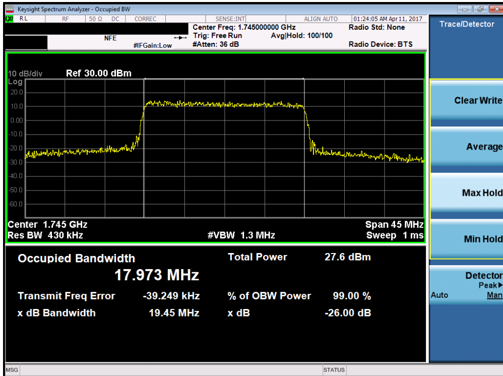
Plot 7-28. Occupied Bandwidth Plot (Band 4/66 – 20.0MHz 16-QAM – RB Size 100)
