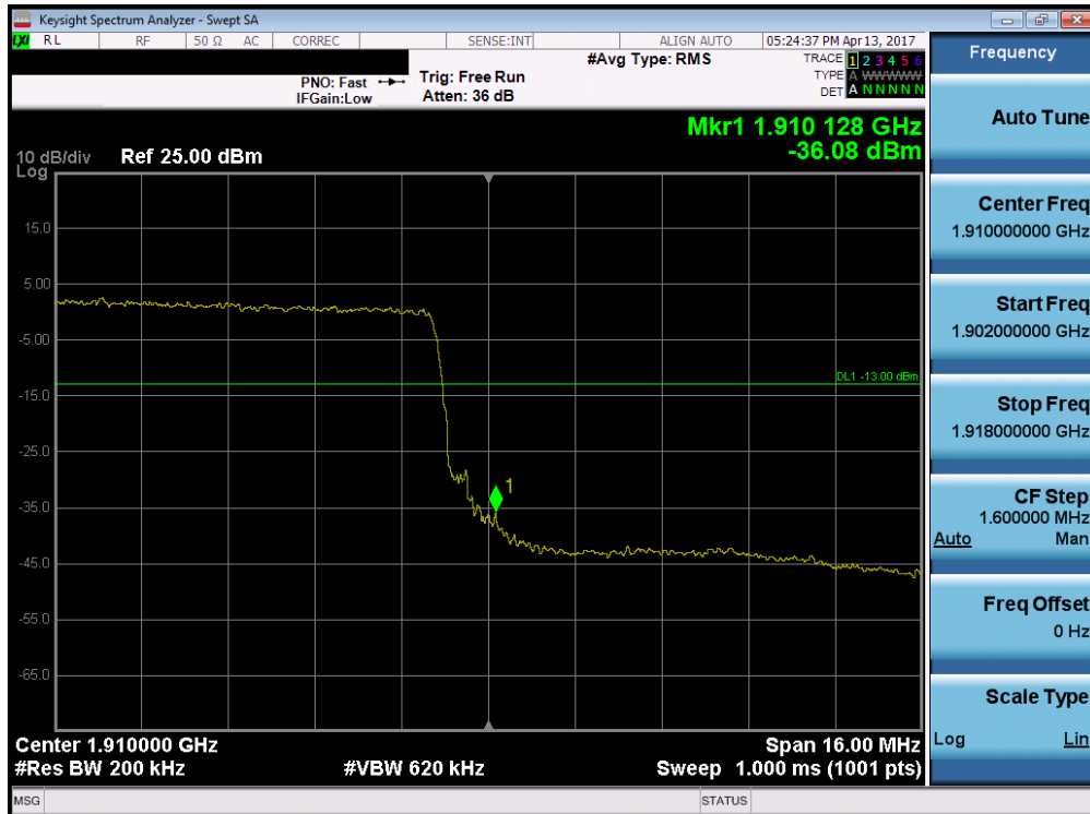
Plot 7-158. Upper Band Edge Plot (Band 2 – 20.0MHz QPSK – RB Size 100)
