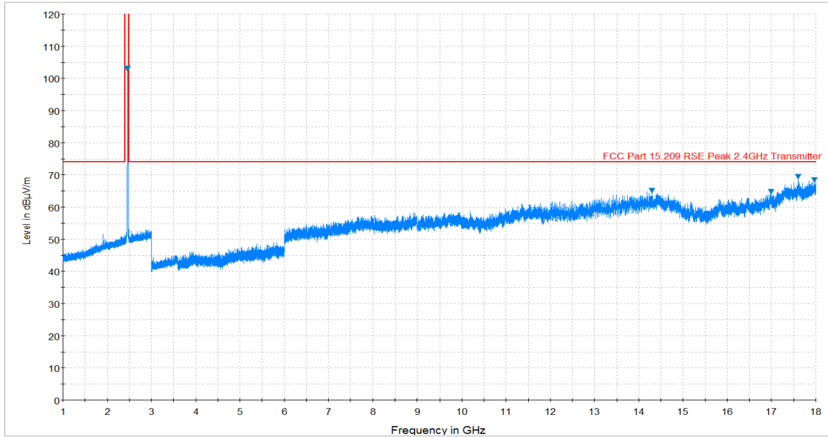
Plot 7-35. Radiated Spurious Plot above 1GHz (802.11b – Ch. 11, Ant. Pol. H)
