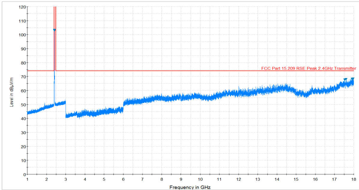
Plot 7-31. Radiated Spurious Plot above 1GHz (802.11b – Ch. 1, Ant. Pol. H)
