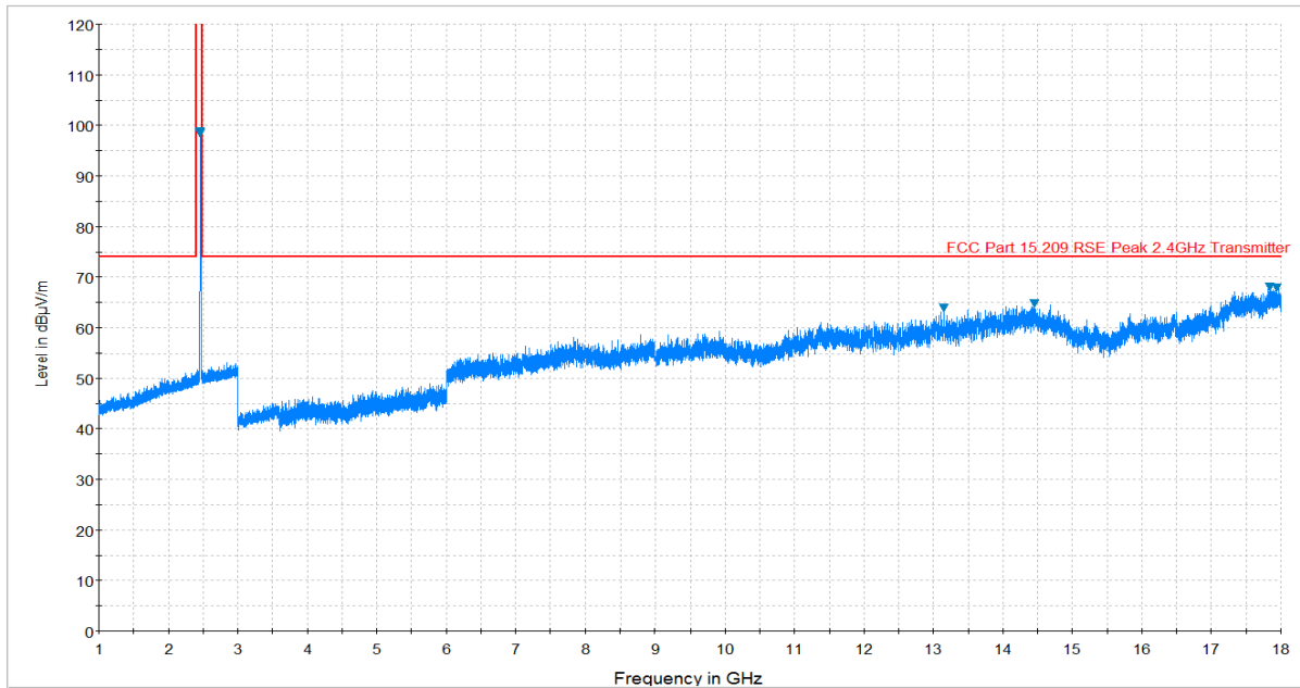
Plot 7-36. Radiated Spurious Plot above 1GHz (802.11b – Ch. 11, Ant. Pol. V)
