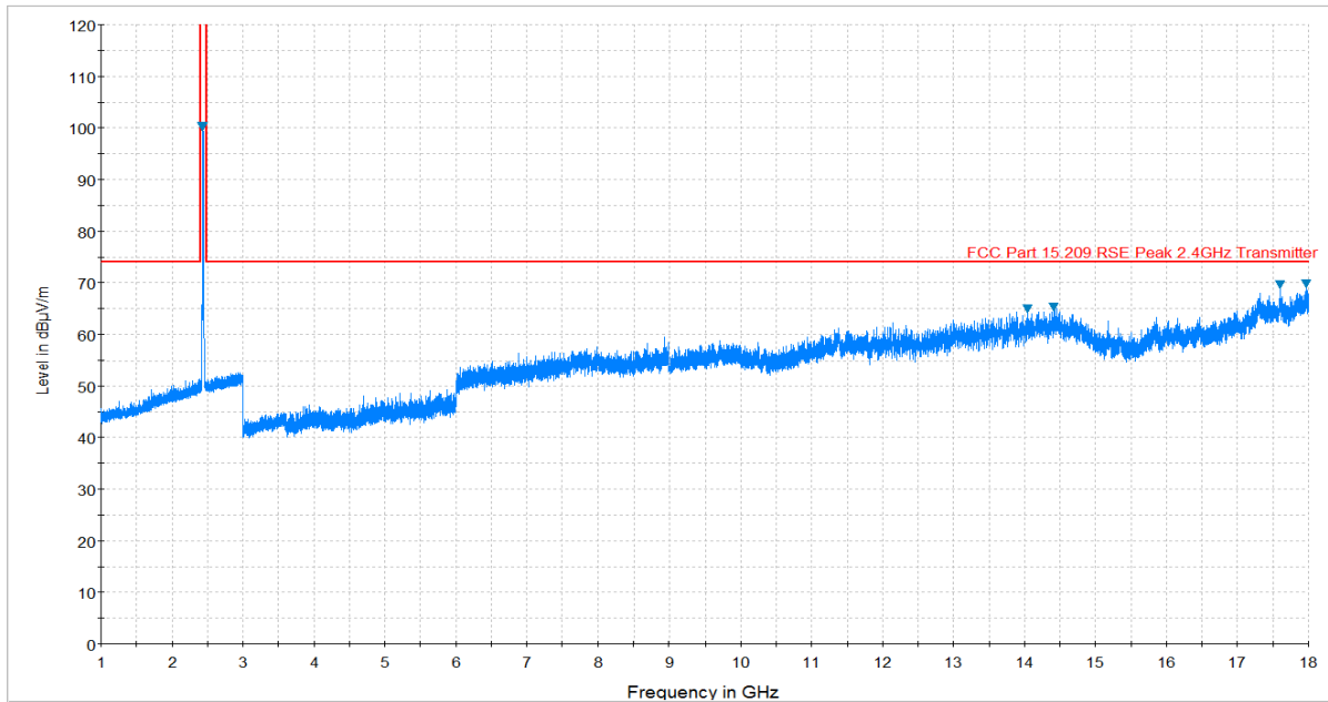
Plot 7-34. Radiated Spurious Plot above 1GHz (802.11b – Ch. 6, Ant. Pol. V)
