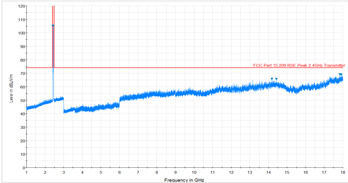
Plot 7-33. Radiated Spurious Plot above 1GHz (802.11b – Ch. 6, Ant. Pol. H)
