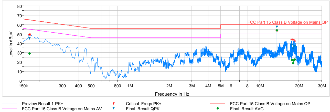
Plot 8-1. Line-Conducted Test Plot with Antenna Connected (L1)
