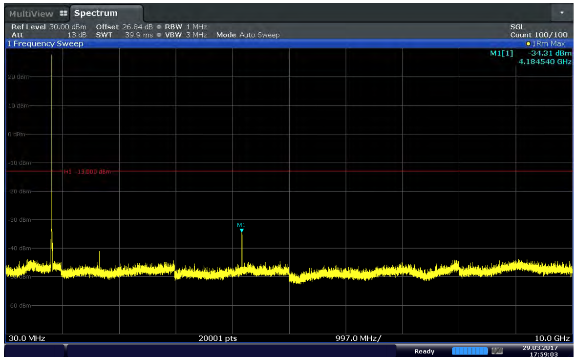
Plot 6-10. Conducted Spurious Plot (Band 5–1.4MHz–QPSK–RB Size 1–RB Offset 5–Ch.20525)
