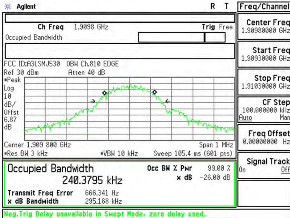
Plot 6-2. Occupied Bandwidth Plot (EDGE1900 Mode - Ch.810)
