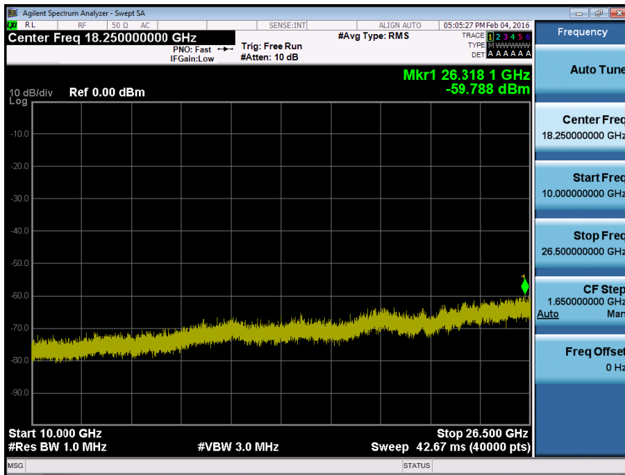
BAND 41. Conducted Spurious Plot 2 (5 MHz Ch. 40265 QPSK RB 1, Offset 0)
