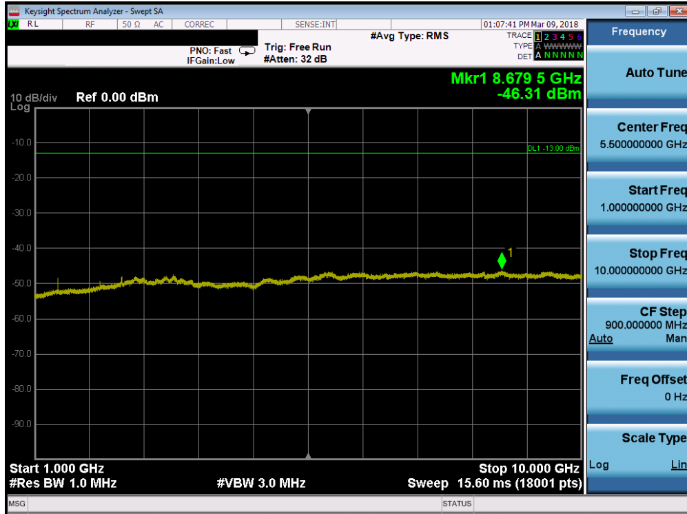
Plot 7-65. Conducted Spurious Plot (Band 71 - 5.0MHz QPSK - RB Size 1, RB Offset 0 - High Channel)
