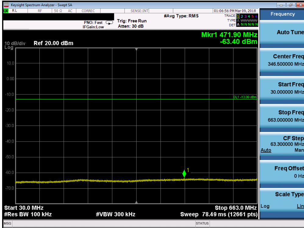
Plot 7-63. Conducted Spurious Plot (Band 71 - 5.0MHz QPSK - RB Size 1, RB Offset 0 - High Channel)
