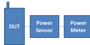
Figure 8-2 Power Measurement Setup for unlicensed modes
