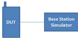
Figure 8-1 Power Measurement Setup for licensed modes
