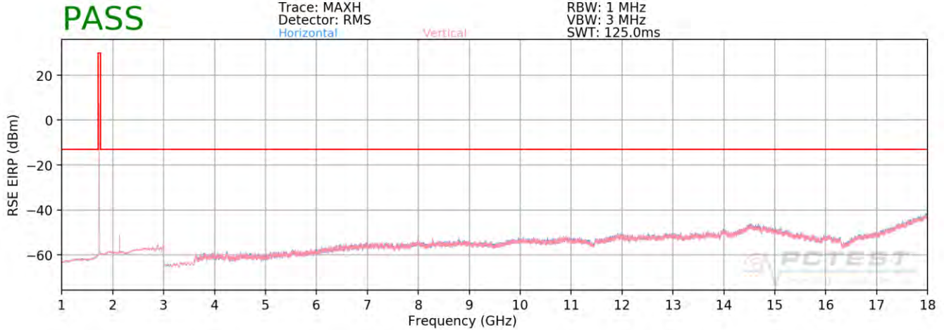
Plot 7-105. Radiated Spurious Plot above 1GHz (AWS WCDMA)
