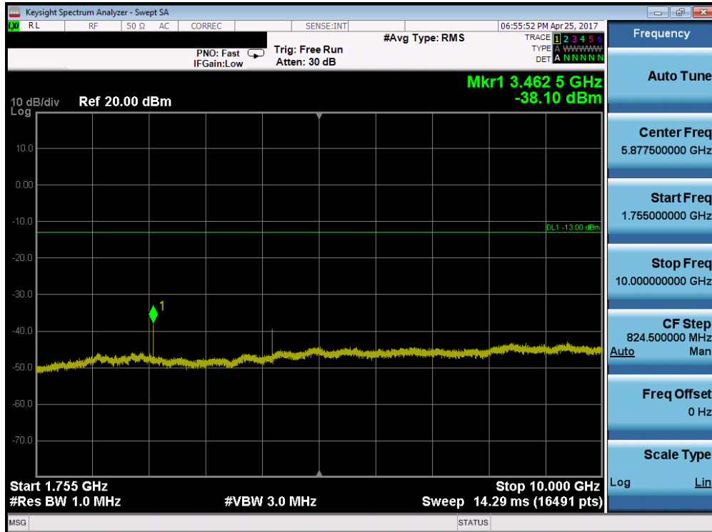
Plot 7-59. Conducted Spurious Plot (Band 4 – 3.0MHz QPSK – RB Size 1, RB Offset 0 – Mid Channel)
