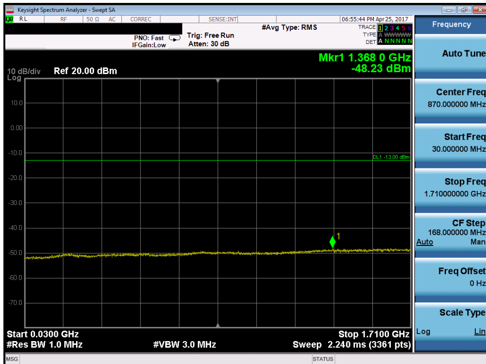
Plot 7-58. Conducted Spurious Plot (Band 4 – 3.0MHz QPSK – RB Size 1, RB Offset 0 – Mid Channel)
