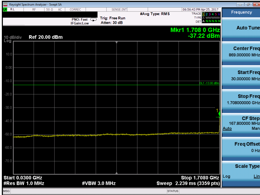
Plot 7-55. Conducted Spurious Plot (Band 4 – 3.0MHz QPSK – RB Size 1, RB Offset 0 – Low Channel)
