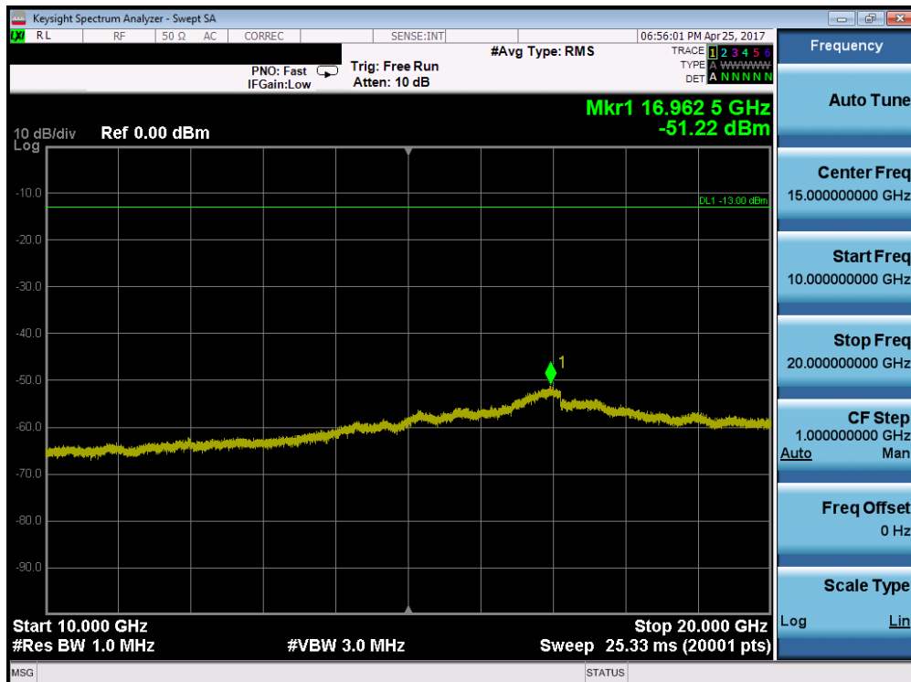
Plot 7-60. Conducted Spurious Plot (Band 4 – 3.0MHz QPSK – RB Size 1, RB Offset 0 – Mid Channel)
