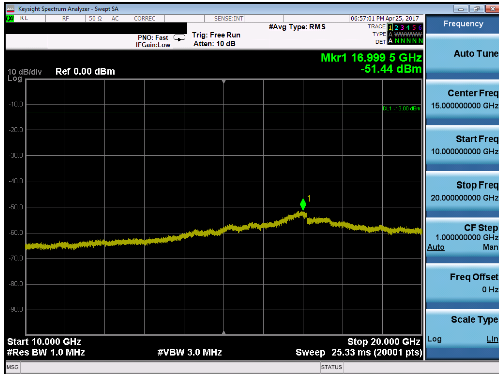
Plot 7-57. Conducted Spurious Plot (Band 4 – 3.0MHz QPSK – RB Size 1, RB Offset 0 – Low Channel)
