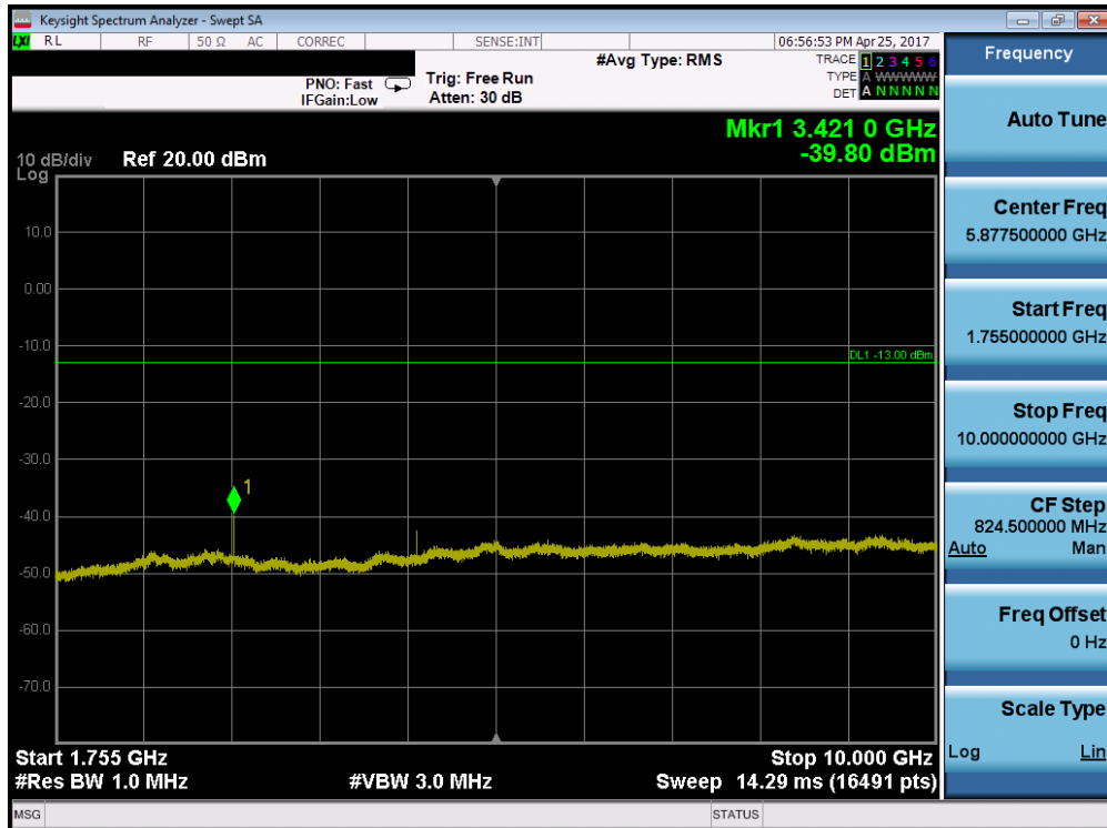
Plot 7-56. Conducted Spurious Plot (Band 4 – 3.0MHz QPSK – RB Size 1, RB Offset 0 – Low Channel)
