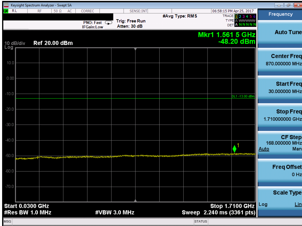
Plot 7-61. Conducted Spurious Plot (Band 4 – 3.0MHz QPSK – RB Size 1, RB Offset 0 – High Channel)
