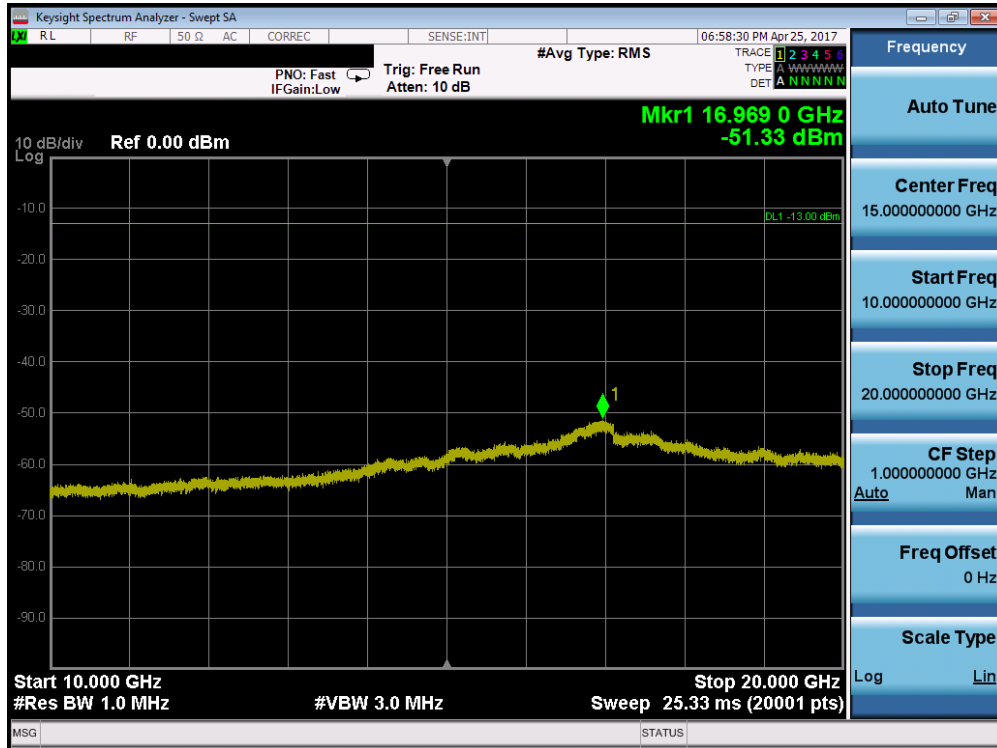
Plot 7-63. Conducted Spurious Plot (Band 4 – 3.0MHz QPSK – RB Size 1, RB Offset 0 – High Channel)
