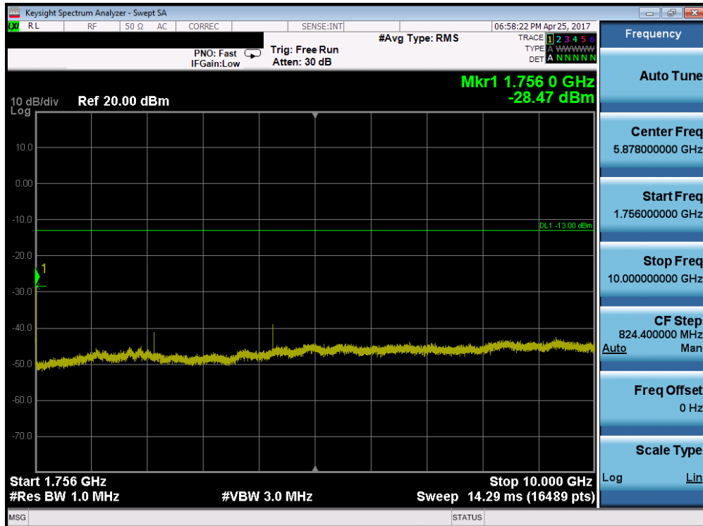
Plot 7-62. Conducted Spurious Plot (Band 4 – 3.0MHz QPSK – RB Size 1, RB Offset 0 – High Channel)
