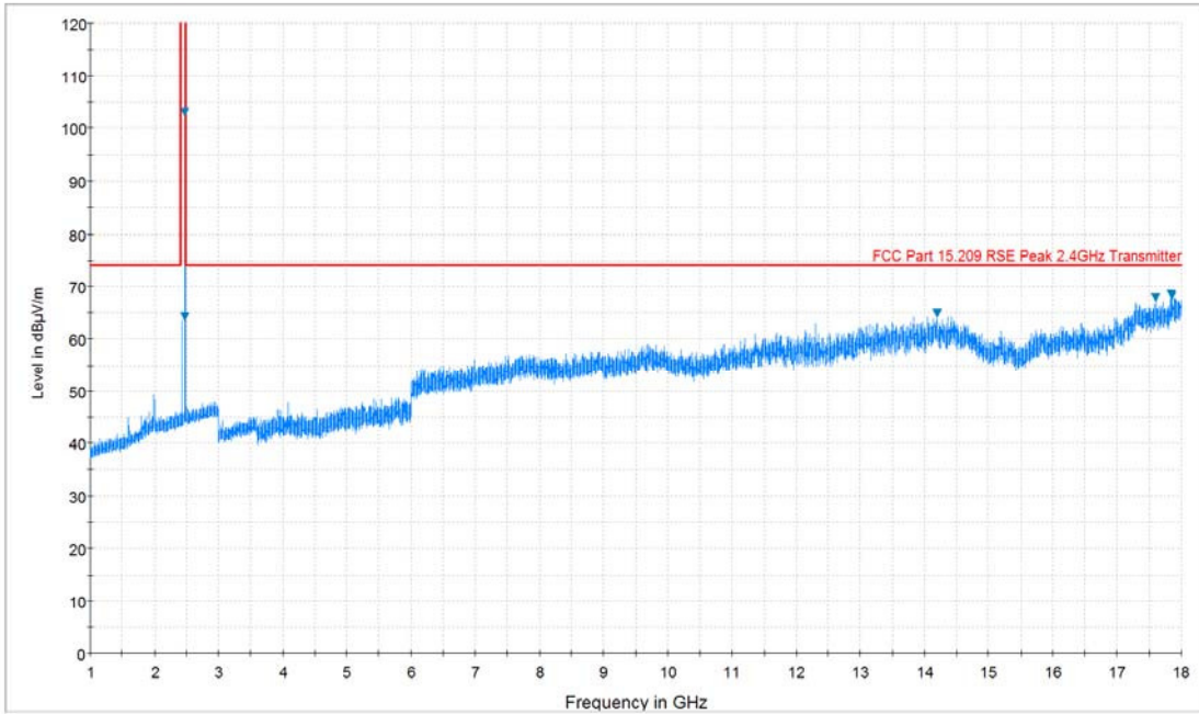
Plot 7-46. Radiated Spurious Plot above 1GHz (BT – Ch. 78, Ant. Pol. H)
