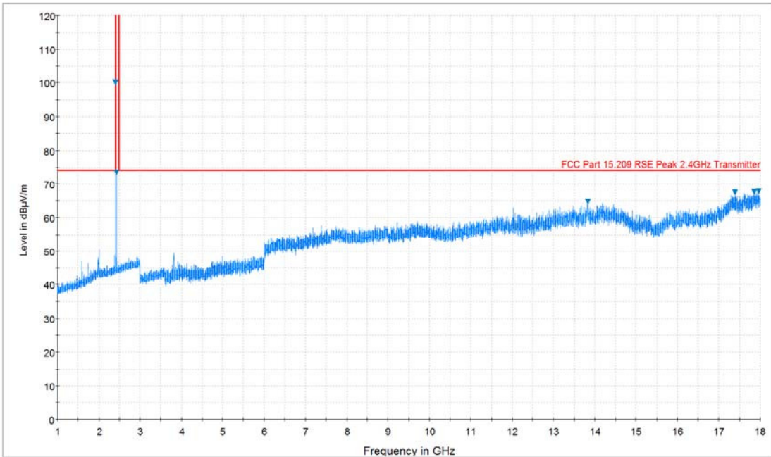
Plot 7-43. Radiated Spurious Plot above 1GHz (BT – Ch. 0, Ant. Pol. V)
