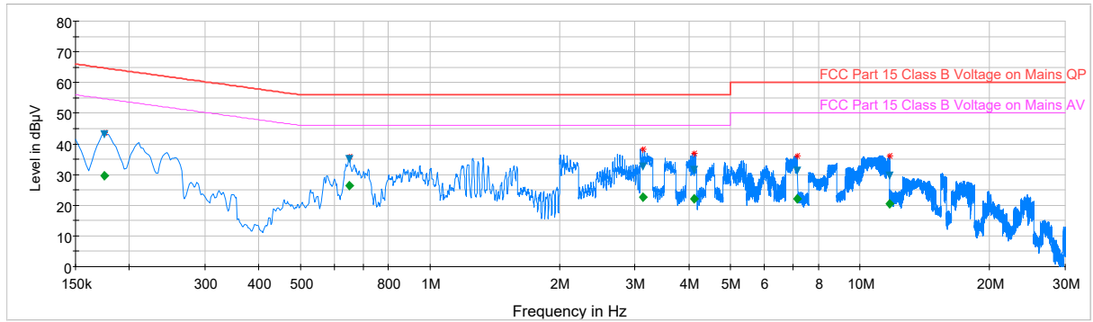
Plot 7-21. Line Conducted Plot with Bluetooth LE (N)
