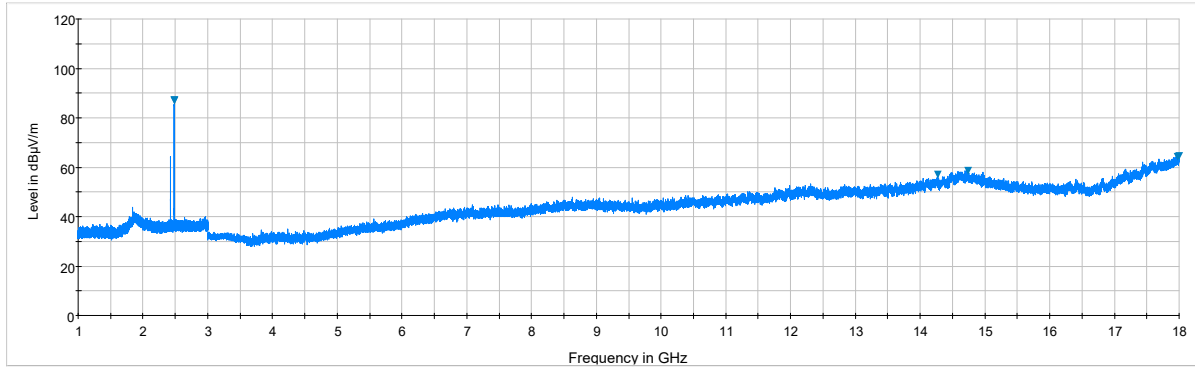
Plot 7-43. Radiated Spurious Plot above 1GHz (BT – Ch. 39, Ant. Pol. V)
