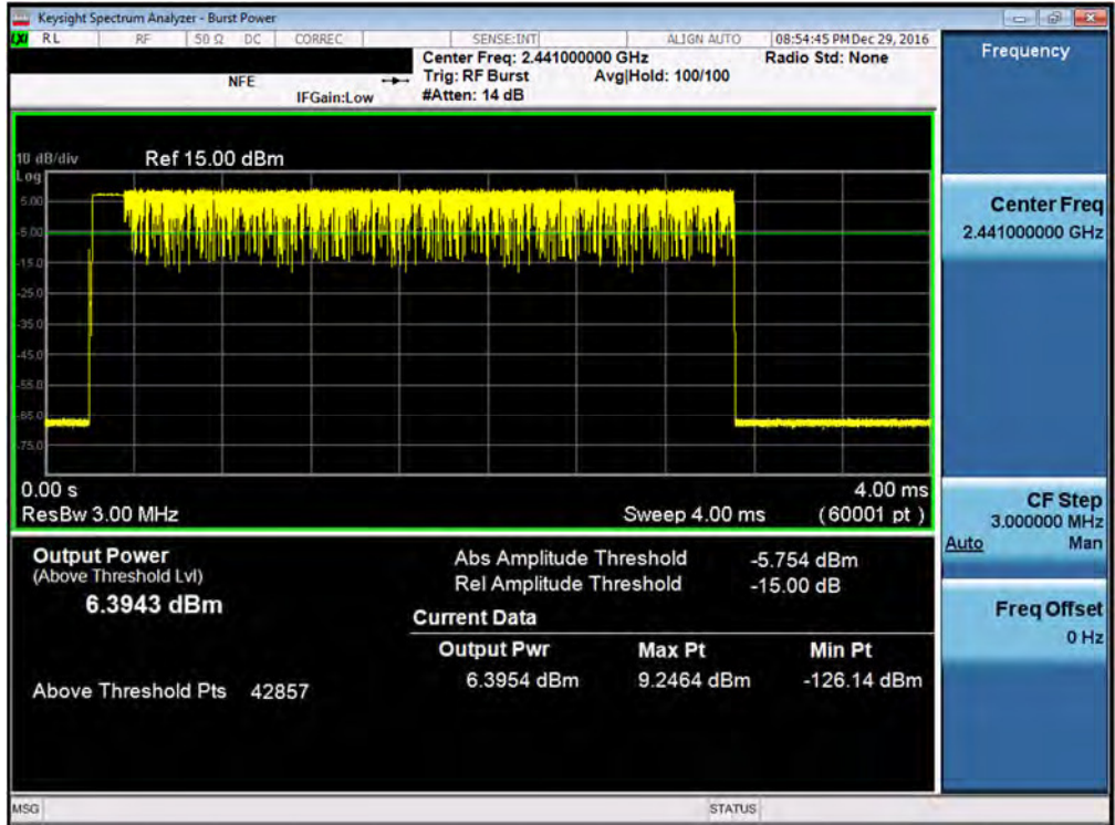
Plot 7-26. Average Conducted Power (3Mbps – Ch. 39)
