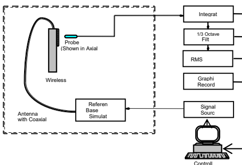
Figure 4-13 Audio Magnetic Field Test Setup
