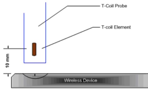
Figure 4-10 Measurement Distance
