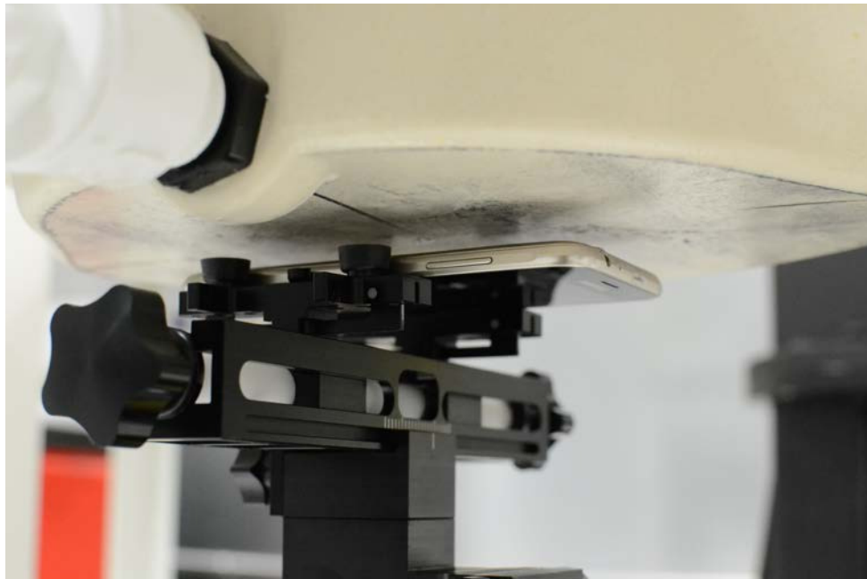
SAR Test Setup Photo 6 – Back Side at 10mm (Hotspot)
