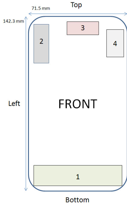
Figure F-1 DUT Antenna Locations
