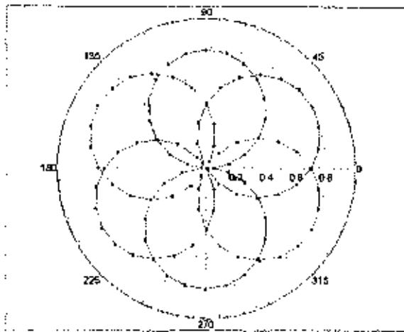
f=600 MHz,TEM
