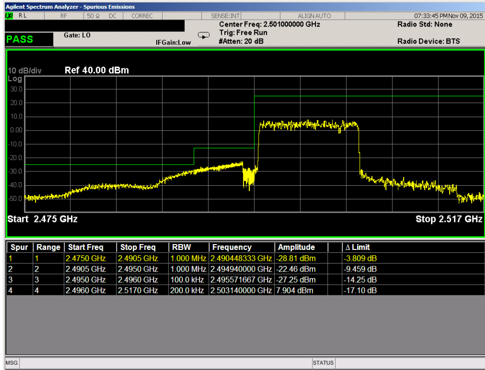
Plot 7-176. Lower ACP Plot (Band 41 – 10.0MHz QPSK – RB Size 50)
